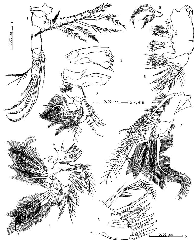
Fig. 3. Longipedia spinulosa n. sp. Female (1-7, holotype; 8, a paratype). 1. antenna; 2. mandible; 3. mandibular praecoxa; 4. maxillula; 5. arthrite of maxillular praecoxa; 6. maxilla; 7. maxillipe; 8. first endite of maxillary syncoxa.
