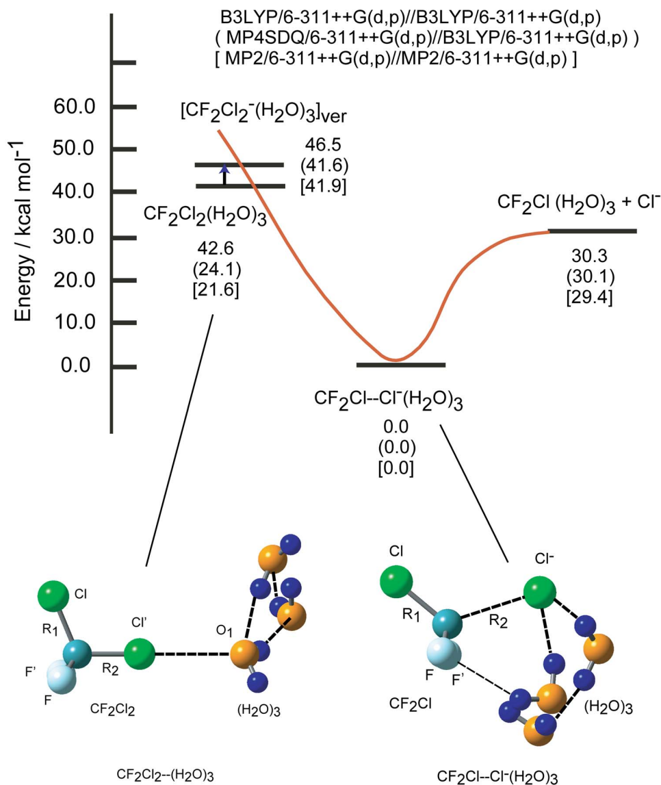
FIG. 3. (Color online) Potential energy diagram for the electron capture process for the CF 2 Cl 2 (H 2 O) 3 system. The optimized structures of neutral and anionic states of CF 2 Cl 2 (H 2 O) 3 are also given.
