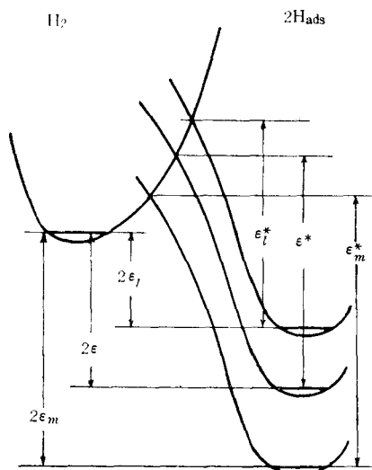
Fig. 1. Potential energy curves involved in the recombination of two adsorbed hydrogen atoms.
