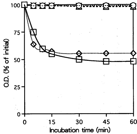
Fig. 3. Germination of heat activated spores (75°C for 20 min) of five strains of Clostridium perfringens type A in K-medium containing KCl (50 mM)+50 mM potassium phosphate buffer (pH 7.0). □: NCTC 8238, ◇: NCTC 8239, ○: HS-13-1, △: S-40, ×: RW-18
