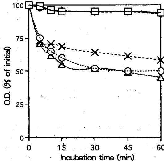
Fig. 4. Germination of non-heated spores of five strains of Clostridium perfringens type A in A-medium containing L-alanine (1 mM)+inosine (1 mM)+CaCl 2 (40 mM)+50 mM Tris-HCl buffer (pH 7.5) in the presence of CO 2 . □: NCTC 8238, ◇: NCTC 8239, ○: HS-13-1, △: S-40, ×: RW-18
