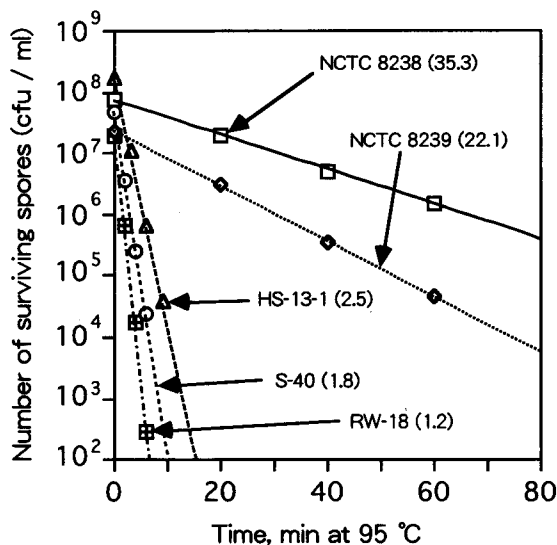
Fig. 1. Thermal survival curves ( D 95 -value) of spores of Clostridium perfringens . Spores were suspended in double distilled water (10 mg dry wt/ml) before measuring the D 95 -value. Numbers in parentheses show D 95 -value.
