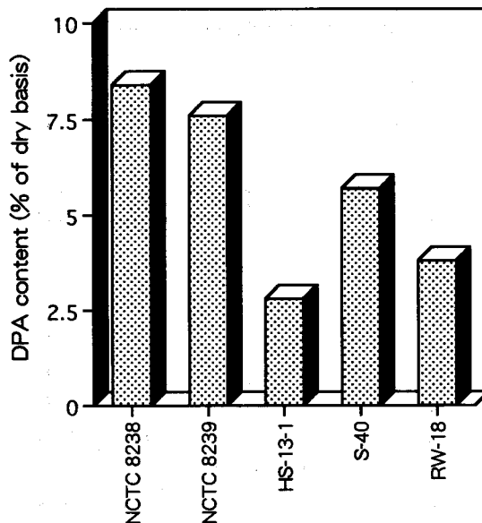
Fig. 2. DPA content in the spores of five strains of Clostridium perfringens type A. DPA content in spores is given by percentage in the spores (dry basis).
