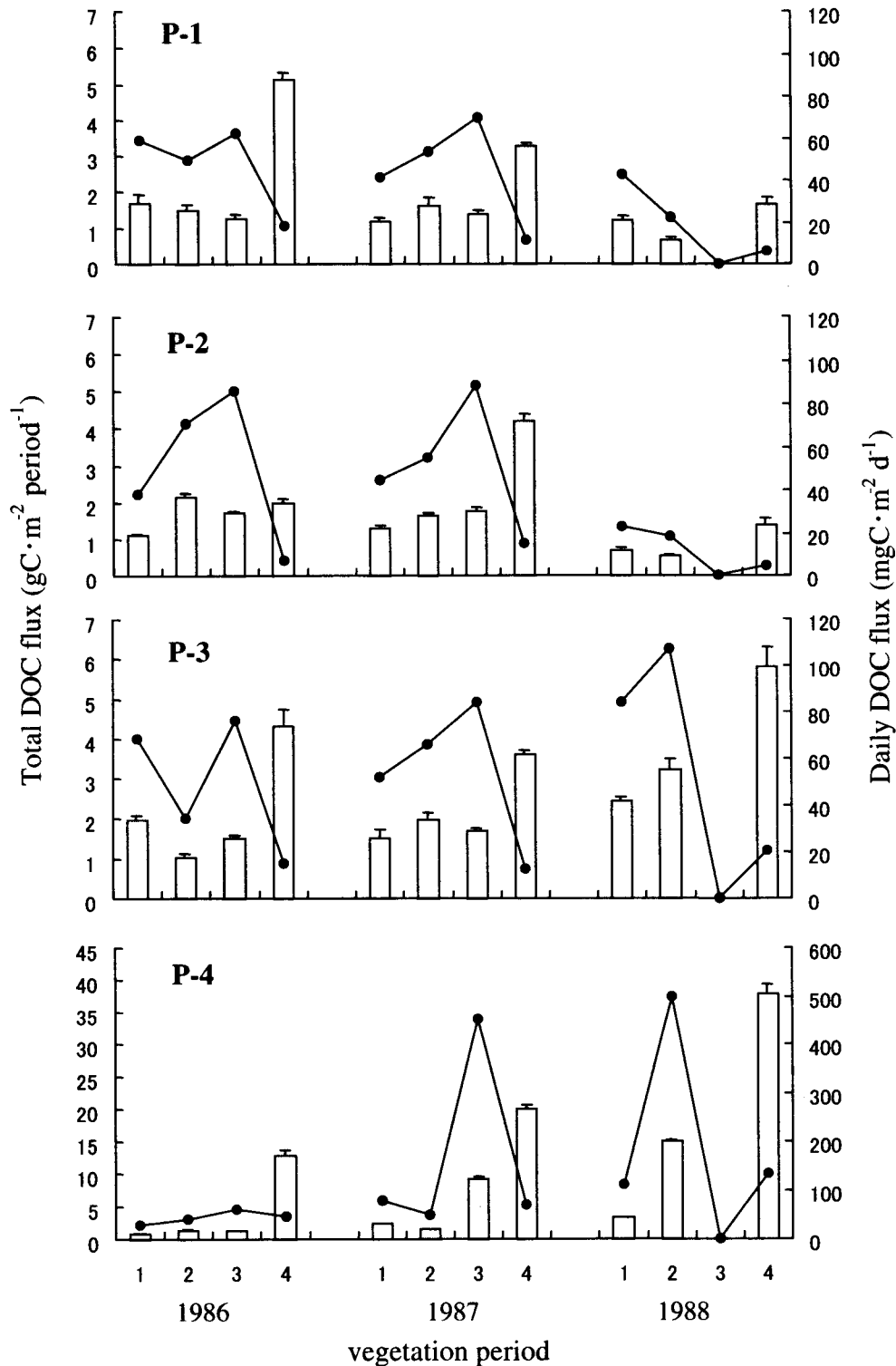
Fig. 10. Seasonal fluctuation of total ( \square ) and daily ( \bullet ) DOC fluxes from the litter layer in each vegetation period in each plot in the pine site using the monthly activated carbon method from 1986 to 1988. Note that the Y-axis of P-4 (bottom) is different from the others. Each bar on the box represents the standard error.
