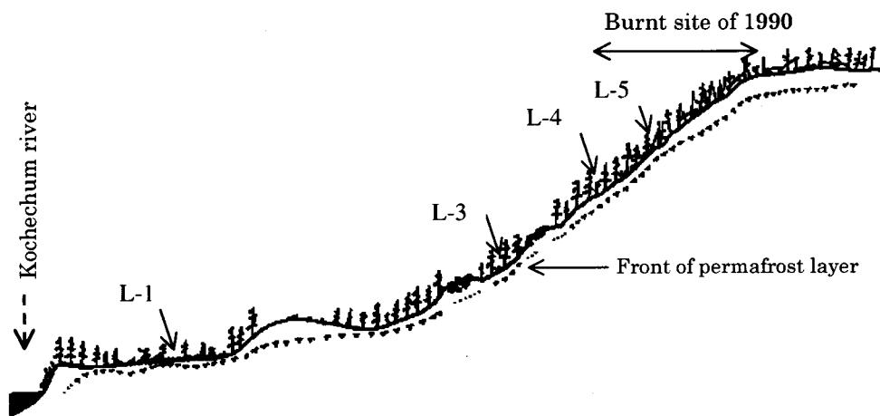
Fig. 2. Locations of studied plots on southwest facing slope in the Larch site, Central Evenkia (Tura) (adapted from Matsuura and Abaimov, 1999)
