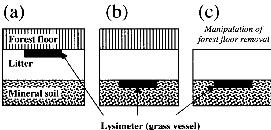
Fig. 4. Locations of lysimeters (glass vessels) under the forest floor (a) and litter (b) at the control site, and under the litter at the experimental removal plot (c).
