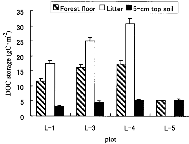
Fig. 7. Extractable DOC storage in the litter at the larch site (July 1998). Each bar on the box represents the standard error.
