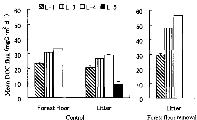
Fig. 5. Daily mean DOC fluxes from the forest floor and litter at the control site (left) and manipulated site (right) in the larch site from July to August 1998. Samples were collected in the glass vessels. There was no forest floor in plot L-5 in the control site. Each bar on the box represents the standard error.
