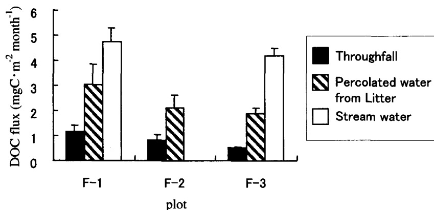
Fig. 13. Mean DOC flux in throughfall, percolated water from litter and stream water in each plot in the fir site from June to September 1992. Stream water was not observed in F-2 plot. Each bar on the box represents the standard error.
