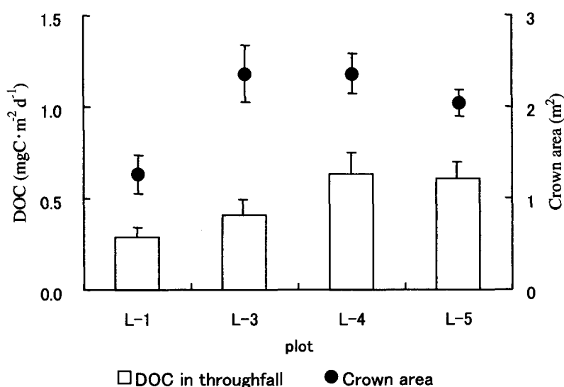
Fig. 6. Daily mean DOC fluxes in throughfall and crown area in each plot in the larch site from July to August 1998. DOC in throughfall was collected using glass vessels. Each bar on the box represents the standard error.
