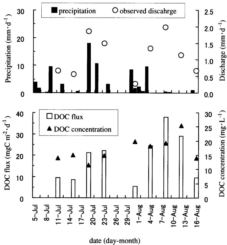
Fig. 8. Daily precipitation, stream discharge (upper), DOC flux and concentration in stream water (lower) at the larch site from July to August 1999.
