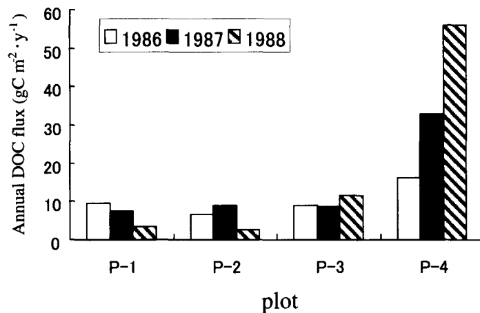
Fig. 11. Annual DOC flux from the litter layer in each plot in the pine site using the monthly activated carbon method from 1986 to 1988. Each bar on the box represents the standard error.
