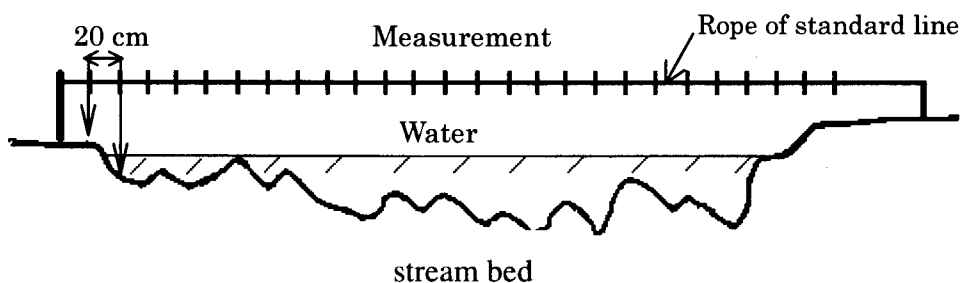
Fig. 3. Scheme of cross-sectional measurements in a stream.
