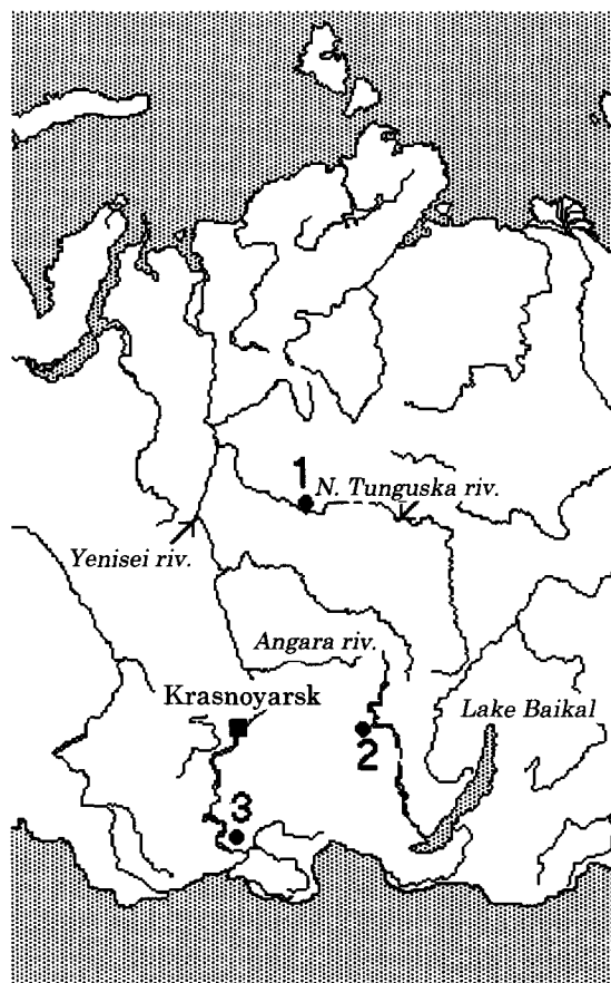
Fig. 1. Location of each study site in central Siberia.
