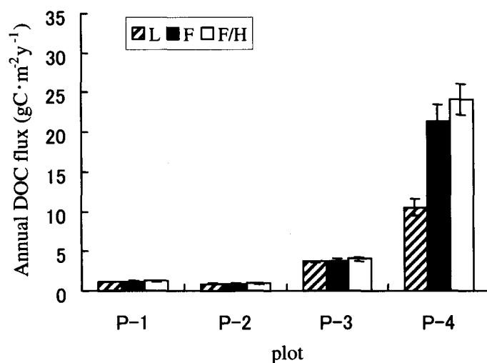
Fig. 12. Annual DOC flux from each layer in the organic horizon in each plot in the pine site using the annual activated carbon method from August 1988 to August 1989. Each bar on the box represents the standard error.
