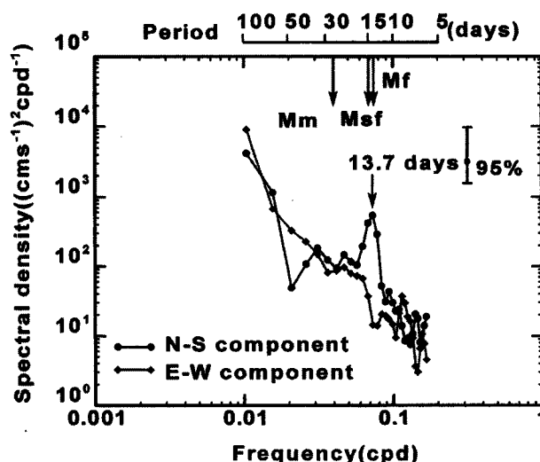
Fig. 10. Power spectral densities of the eastward (diamond) and northward (solid circle) component average flow velocity data at Stns. 5–11 in 48 m depth.
