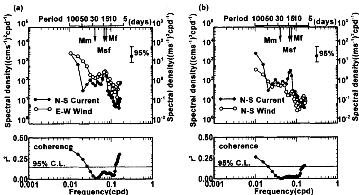
Fig. 13. Cross-spectral-coherence between the 3-day mean value of north-south component of mean current and that of long-strait (east-west component) wind data, power spectral densities (upper), and coherence-squared (bottom) (a). Coherence between the 3-day mean value of north-south component of mean current and that of cross-strait (north-south component) wind data (b).
