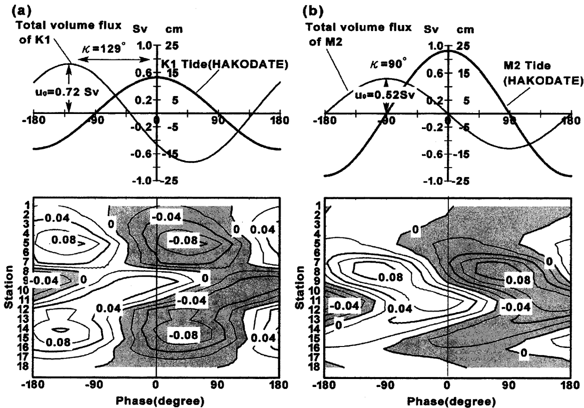
Fig. 7. The relation between the tide of Hakodate and the vertical integrated volume transport of the tidal current in the Strait (K1 (a) and M2 (b)). Sinusoidal variations of the total volume transport of the tidal current to the maximum tide of Hakodate (upper panels), and space-phase diagrams of the vertical volume flux to the phase of the Hakodate tide (lower panels). Contours give transport in 0.02 Sv. The shaded area indicates negative (westward) transport (the tidal current directs to the Japan/East Sea).
