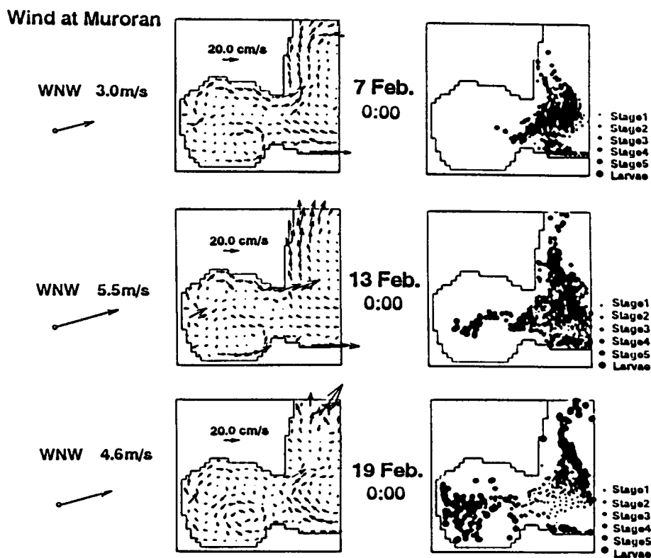
Fig.1. Instantaneous fields of the calculated current vectors(left panel), and the horizontal distributions of modeled walleye pollock eggs/larvae(right panel) at the intervals of six days.
