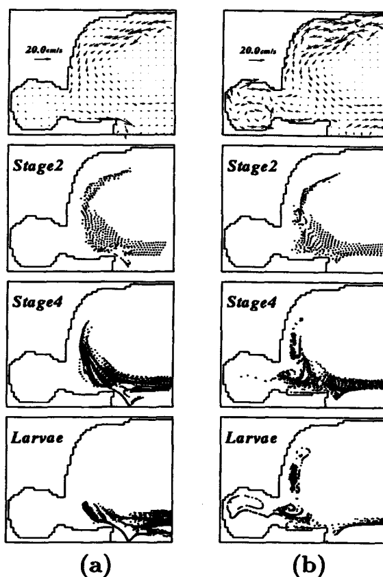
Fig.2. (a) Horizontal distributions of current field and modeled eggs/larvae under the constant inflow-outflow condition calculated by single layer model after 30 days. Model forcing term is only 0.5sv inflow-outflow condition. (b) The same as (a), but model forcing terms of both wind and inflow-outflow conditions. The northwesterly(from left to right in figure) wind, which has constant wind velocity(10m/s), is blowing.
