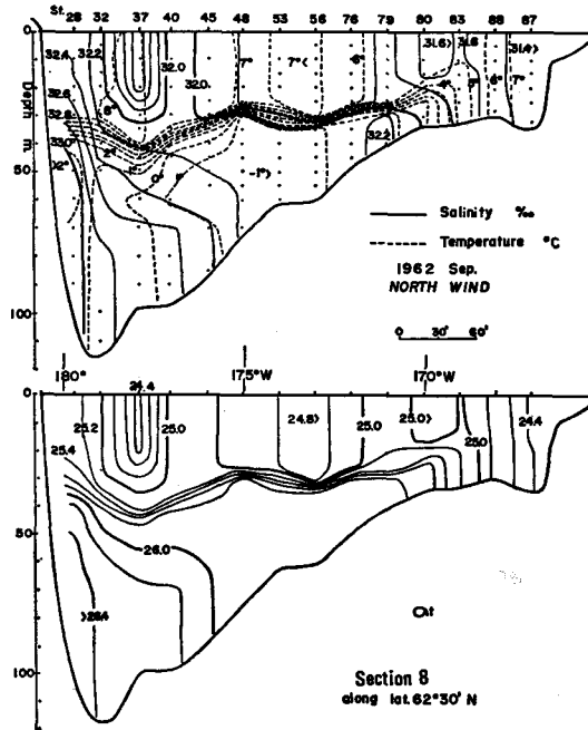
Fig. 35. Vertical sections of temperature, salinity and \sigma_t at the entrance of the Gulf of Anadair. Locations of Sections are shown in Fig. 29.
