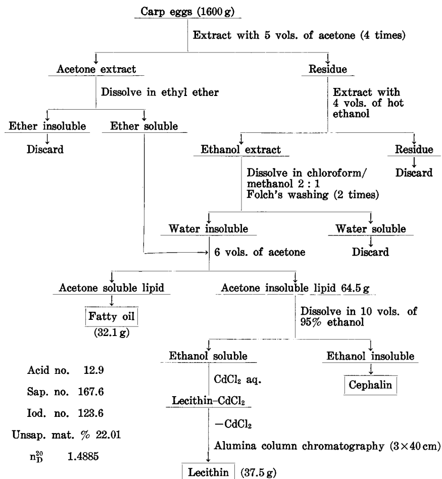
Fig. 6. Extraction and Fractionation of the Lipids from Carp Eggs
