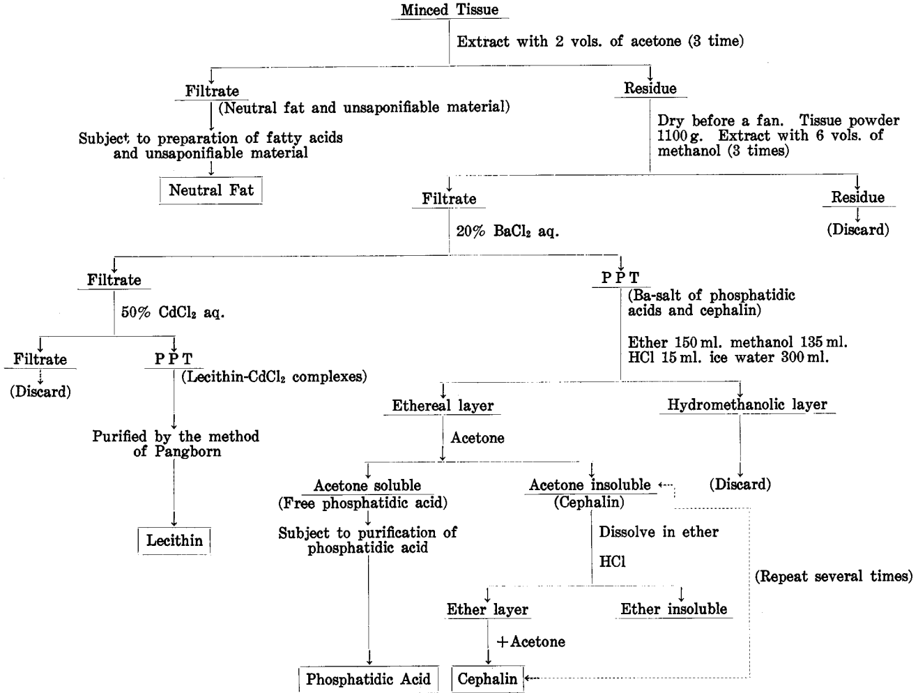
Fig. 7. Extraction and Purification of the Phospholipids from Rorqual Heart
