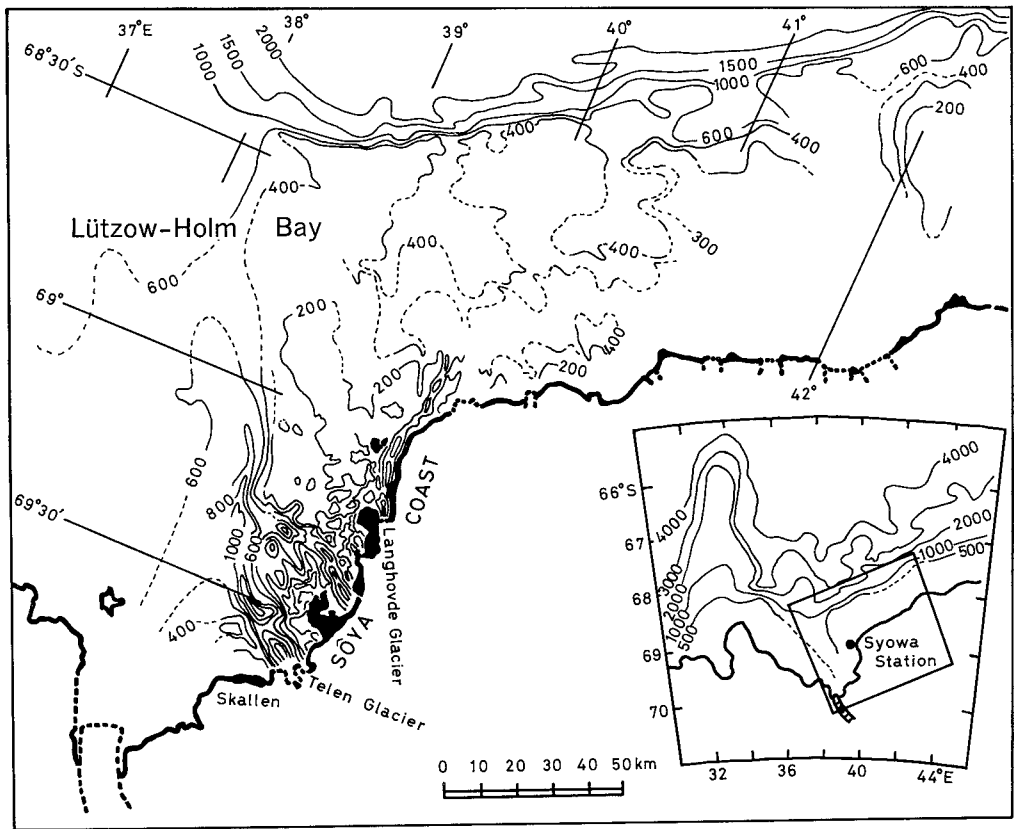
Fig. 1 Bathymetry of Lützw-Holm Bay.
