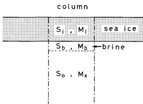
Fig. 20 An imaginary distribution as the result of the freezing of seawater in a water column with the same cross-sectional area as the sampler. Details in the text.
