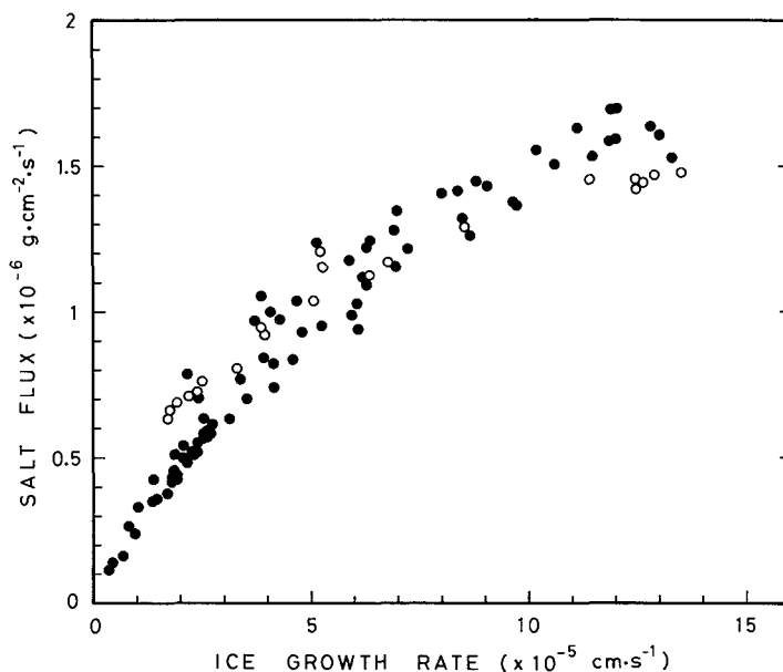
Fig. 35 Comparisons of salt flux between values (○) obtained by brine collection and values (●) estimated from sea ice salinity.
