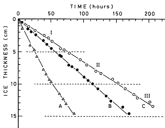
Fig. 24 Ice thickness vs. time of measurement at three constant ice growth rates, 0.170 (A), 0.086 (B) and 0.064 (C) \text{cm} \cdot \text{h}^{-1} . Stages I, II, III show the first, the second, the third period during which brine was collected.
