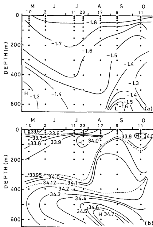
Fig. 6 Seasonal variations in (a) water temperature (°C) and (b) salinity (‰) profiles in the Ongul Strait.
