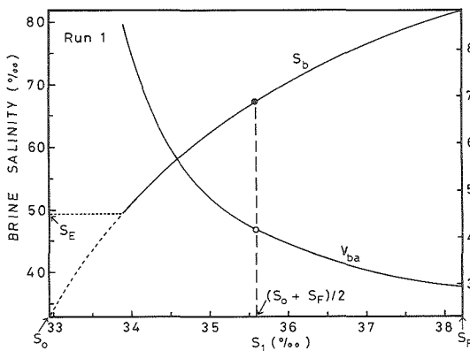
Fig. 27 Effect of change in S_1 on S_b and V_{ba} (run 1).
