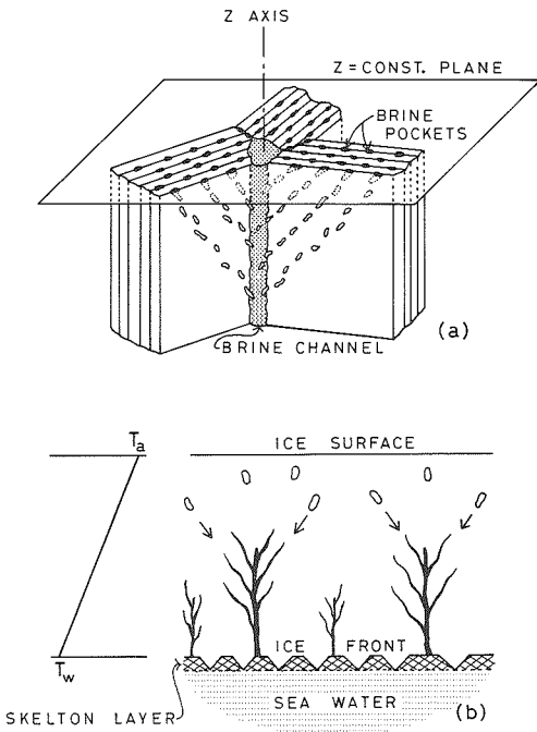
Fig. 8 Schematic diagrams of sea-ice structure. (a) Microscopic drawing of ice crystals, brine pockets and a brine drainage channel ; (b) macroscopic vertical section of tree-shaped channels, T_a and T_w representing air and seawater temperatures, respectively, where T_a < T_w .
