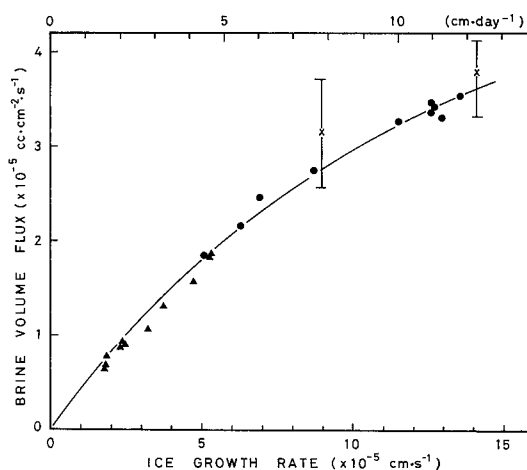
Fig. 30 Volume flux of brine vs. ice growth rate. Circle, field data; triangle, laboratory data; cross, data obtained by analyzing schlieren movie films (bar indicates a limited analysis of the movie films).
