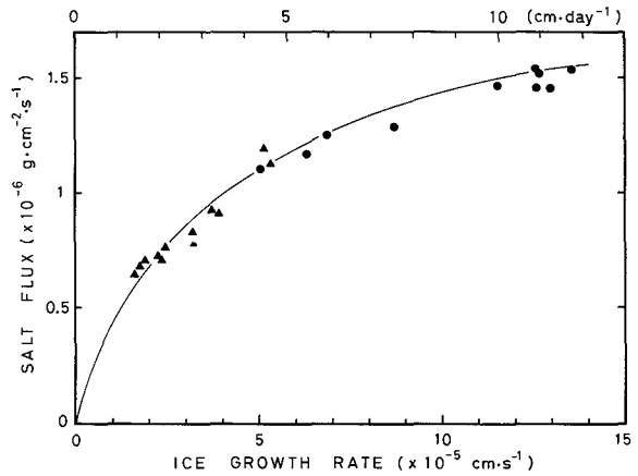
Fig. 31 Salt flux of brine vs. ice growth rate. Circle, field data; triangle, laboratory data.
