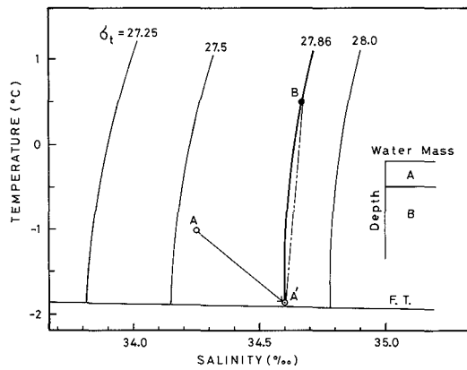
Fig. 7 Temperature-salinity diagram. F. T., equilibrium line of freezing temperature. Details in the text.
