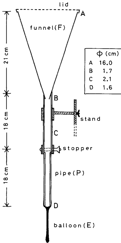
Fig. 21 Illustration of the brine sampler used.
