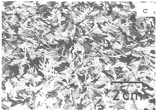
Fig. 10 Horizontal sections of sea ices at the depth of 2.2 cm formed at growth rates : (a) 0.185 \text{ cm} \cdot \text{h}^{-1} , (b) 0.33 \text{ cm} \cdot \text{h}^{-1} and (c) 0.49 \text{ cm} \cdot \text{h}^{-1} .
