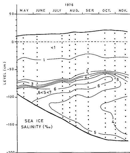
Fig. 5 Seasonal variations in sea-ice salinity profiles in the Ongul Strait. The broken line represents the sea level, and the dots indicate locations of ice samples collected.
