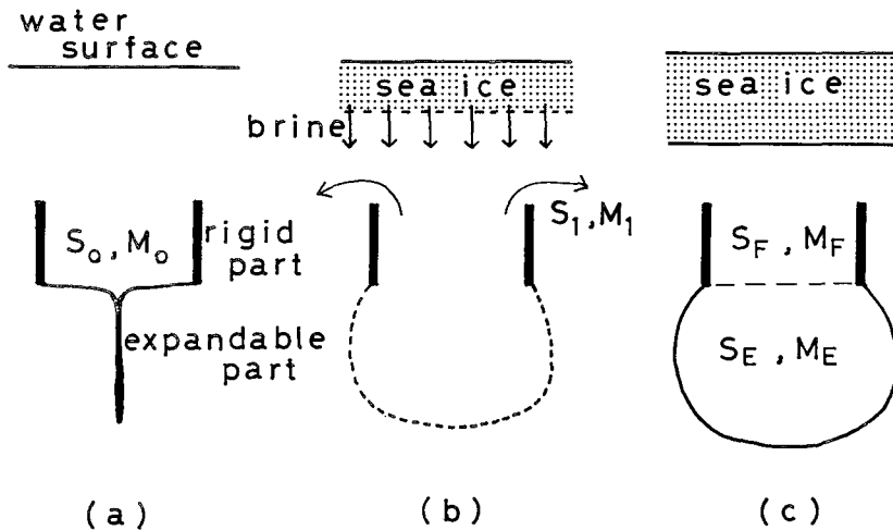
Fig. 19 Modeling on a possible phenomenon which may occur in the sampler while brine is being collected (a) at the start of surface freezing, (b) during the freezing period and (c) at the finish of the collection. Details in the text.
