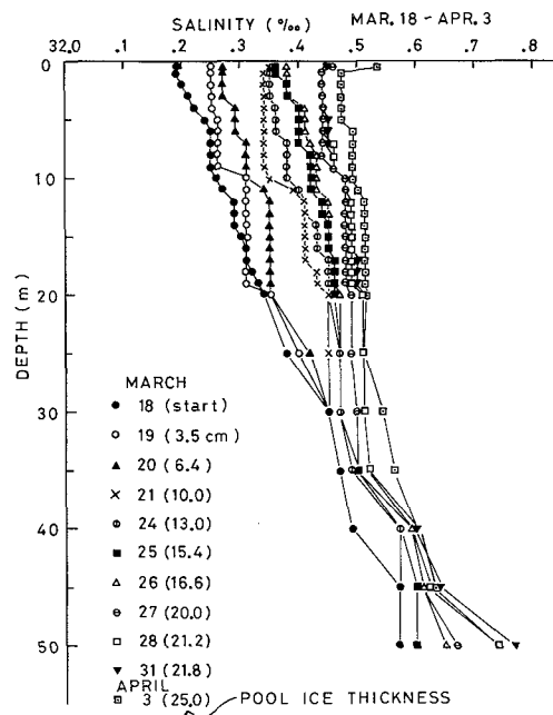
Fig. 3 Change in water-salinity profiles under growing sea ice in the pool.
