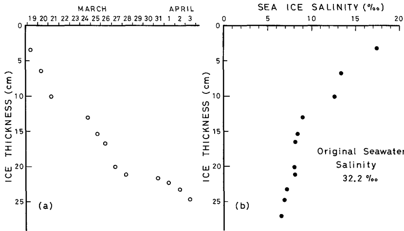
Fig. 2 Ice thickness vs. date of measurement (a) ; Bulk ice salinity vs. thickness (b).
