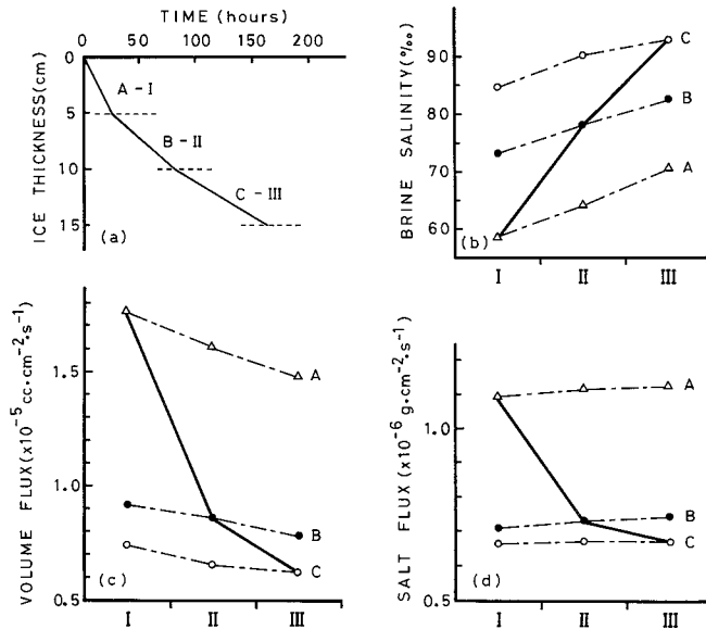
Fig. 33 Changes in (b) salinity, (c) volume flux and (d) salt flux of brine with (a) a hypothetical process of ice growth. Various marks correspond to those indicated in Figs. 24 or 32. Details in the text.
