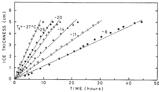
Fig. 9 Change in sea ice growth rate with air temperature ( T_a ).
