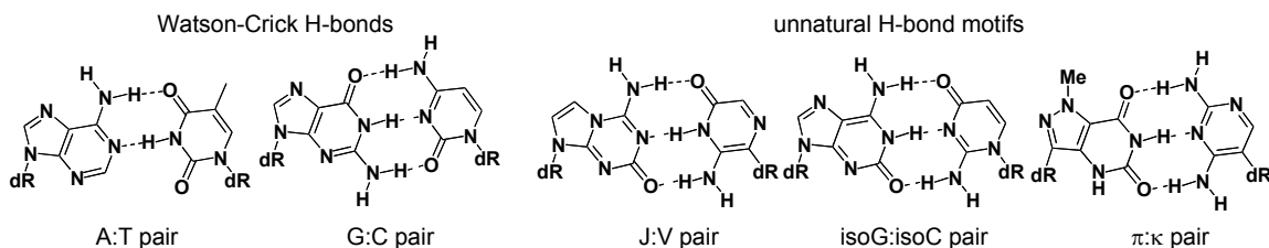
Figure 1. Watson-Crick hydrogen-bonds and examples of unnatural hydrogen-bonds
