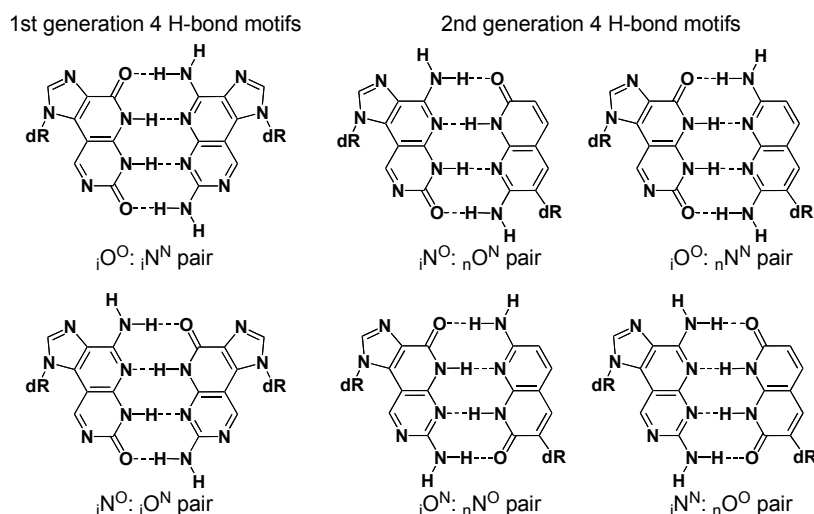
Figure 2. Four hydrogen-bonding motifs
