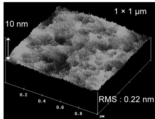
Fig. 3. Three-dimensional AFM image ( 1 \times 1 \mu\text{m} ) of the surface topography of a 50-nm-thick CMS thin film annealed at 600^\circ\text{C} after deposition.
