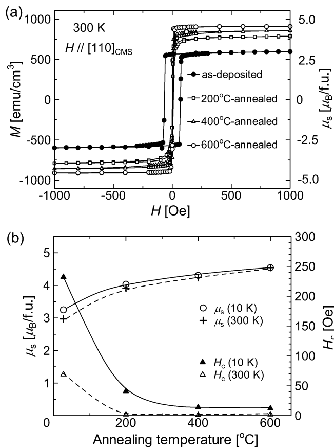
Fig. 4. Magnetic properties of CMS films. (a) Magnetic hysteresis curves up to 1000 Oe at 300 K for 50-nm-thick CMS films as-deposited and postdeposition annealed at 200–600 °C. The magnetic field was applied along the [110]_{\text{CMS}} axis. Magnetization due to the substrate has been subtracted. (b) Annealing temperature dependence of the saturation magnetization, \mu_s , and the coercive force, H_c , for 50-nm-thick CMS thin films.
