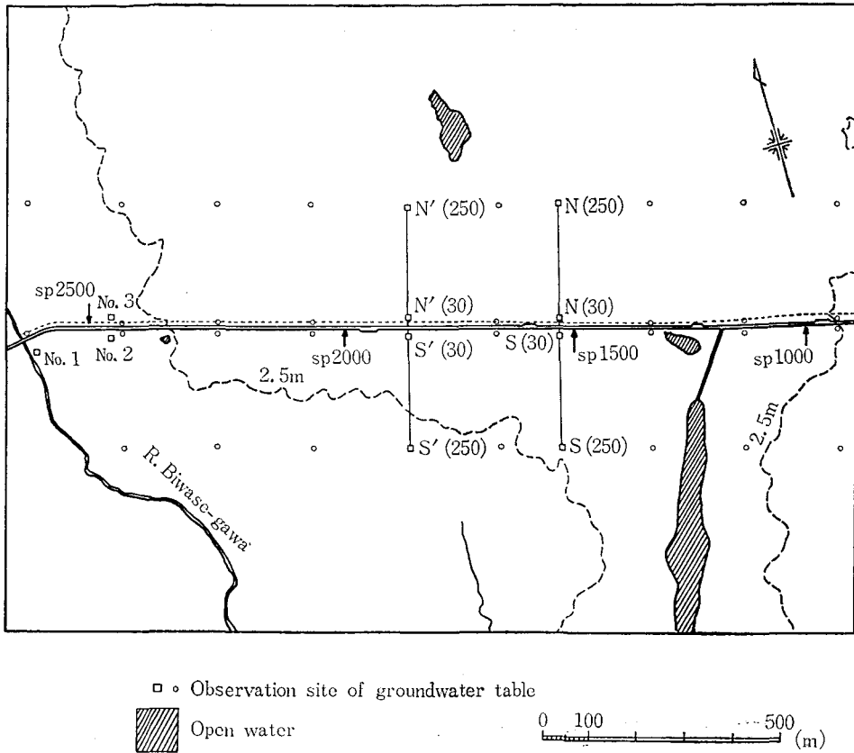
Fig. 2. Location of observation lines and groundwater table recorder.
