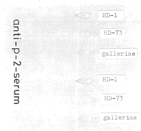
Fig. 10. Crossed immunoelectrophoresis of dissociated crystals against anti-P-2-serum in the subsp. galleriae . An increased volume of anti-serum ( 450 \mu\text{l} ) was added to the agarose gel.
