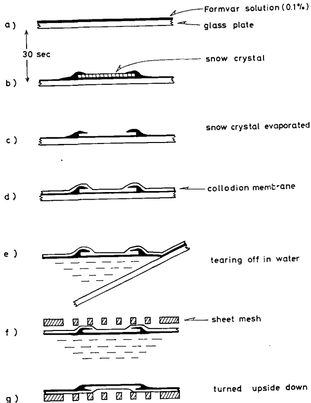
Fig. 1 Replication process by sandwich technique.
