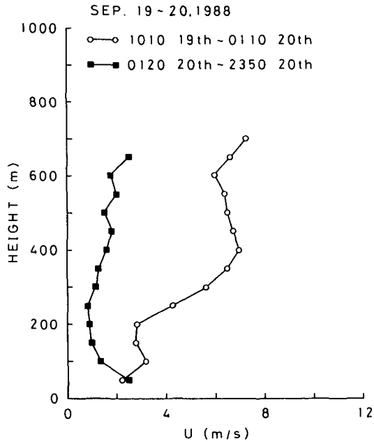
Fig. 5. Profile of averaged horizontal wind speed from 1010 JST, 19 Sep. to 2350 JST, 20 Sep., 1988. \circ : before the passage of the front (1010 19th-0110 20th). \blacksquare : after the passage of the front (0120-2350 20th).
