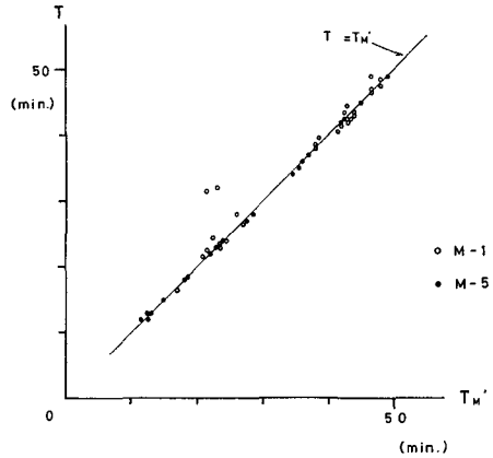
Fig. 20 Comparison between the period estimated by the general formula ( T_{M'} ) and that obtained by the numerical calculation ( T ).
