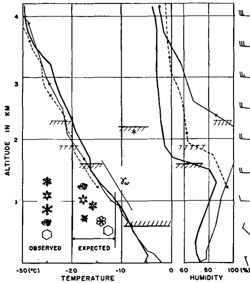
Fig. 16 Vertical distribution of temperature, humidity and wind. Types of snow crystals, observed and expected, 19 Feb. 1964.
