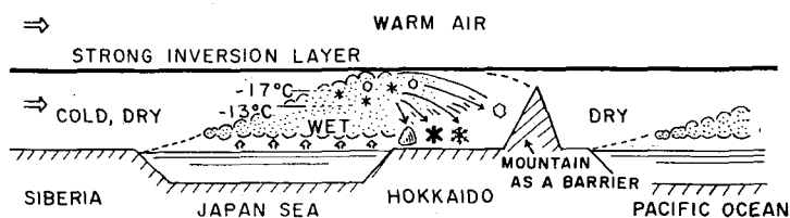
Fig. 20 Proposed model of mechanism for snowfall of low land type in winter monsoon season.
