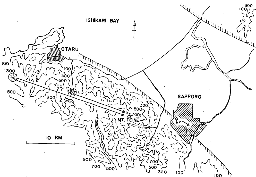
Fig. 7. Horizontal trajectories of falling snow crystals and radio sonde balloon.
