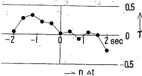
Fig. 9. Correlation between E_1(t) and E_{10}(t+n\Delta t) . n\Delta t > 0 means that E_1 is advancing in phase to E_{10} . t=40 sec. interval = 0.40 sec.
