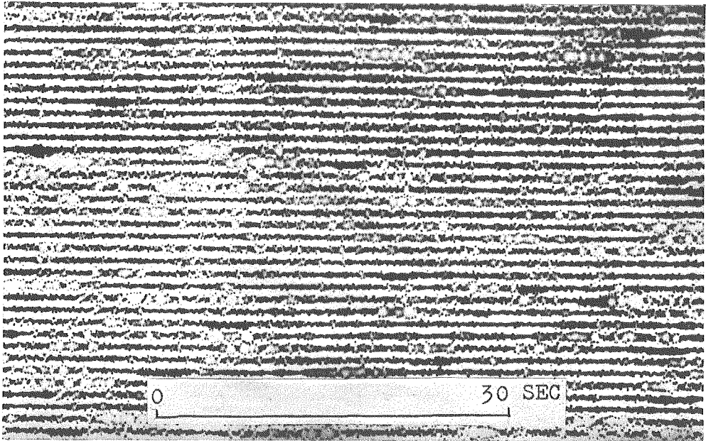
above: New craters, seen from western wall of old crater (June 16, 1956). below: Tremor at Station No. 1 (August 3, 1956).
