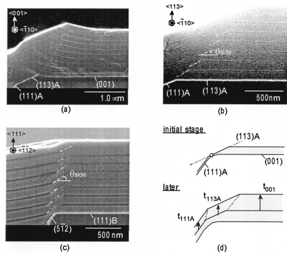
FIG. 3. Cross-sectional SEM images of samples after repeated growth of AlGaAs (100 nm)/GaAs (10 nm) on basic one-sided mesa: (a) \langle -110 \rangle -oriented mesa on a (001) substrate; (b) \langle -110 \rangle -oriented mesa on (113)A substrate, and (c) \langle -1-12 \rangle -oriented mesa on a (111)B substrate. (d) A likely mechanism for evolution of the (113)A facet for growth on (001) substrate.
