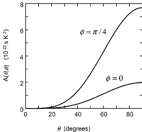
FIG. 2. Angular dependence of the coefficient A of the attenuation rate in the (100) ( \phi=0 ) and (110) ( \phi=\pi/4 ) planes of \text{TeO}_2 .
