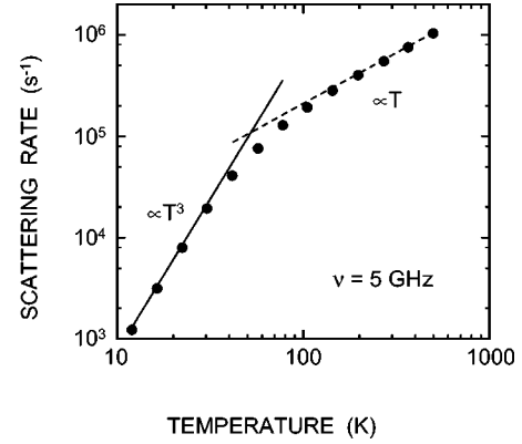
FIG. 3. Temperature dependence of the attenuation rate of L phonons of frequency 5 GHz propagating in the [110] direction. The solid circles are the results of numerical calculations based on Eq. (13). The solid line is the analytical result [Eq. (29)] for low temperatures and the dotted line is the high temperature formula [Eq. (36)].
