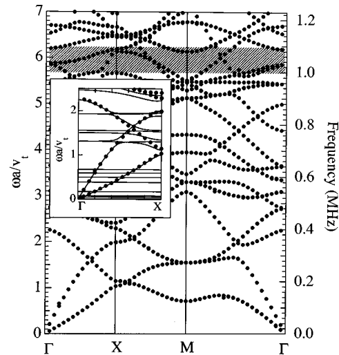
FIG. 3. FDTD results (with a grid of n\times n=120^2 points in a unit cell) for the dispersion relations of the mixed modes (coupled longitudinal and transverse acoustic waves) in a two-dimensional square lattice consisting of mercury circular cylinders in an Al substrate with filling fraction f=0.4 . ( v_t=3.11\times 10^5 cm/s is the transverse sound velocity in Al and a is the lattice spacing.) Hatched region is the frequency range where large transmission dips are observed for the longitudinal sound (Ref. 6). Inset compares the frequencies obtained by the FDTD calculation (dots) and the PWE method (solid lines) with N\times N=11^2 plane waves in the \Gamma -X direction.
