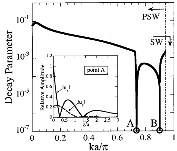
FIG. 8. Decay parameter \epsilon of the pseudosurface waves (PSW's) along the \Gamma -X direction. For the value of k at which \epsilon vanishes (point A), PSW becomes a true surface wave (secluded supersonic surface wave). At point B, PSW is degenerate to the bulk transverse wave propagating along the surface. The lattice displacements vs distance from the surface at point A are plotted in the inset.
