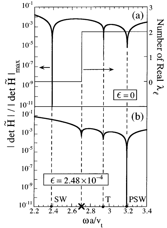
FIG. 7. The normalized magnitude of the boundary condition determinant |\det \tilde{H}| vs frequency along the dot-dashed line ( ka/\pi=0.857 along the \Gamma -X direction) in Fig. 1. (a) For the real wave vector parallel to the surface, with \epsilon=0 . (b) For the complex wave vector parallel to the surface, i.e., \epsilon=2.48 \times 10^{-4} . The frequencies at which the four branches intersect the dot-dashed line (Fig. 1) are labeled. (The cross indicates the frequency at which the dashed line of Fig. 1 intersects the dot-dashed line.) The number of real \lambda_i (the wave number normal to the surface) is also shown in (a).
