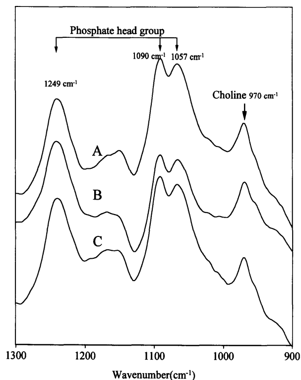
Fig 3. Infrared spectra of phospholipids in range of phosphate head and choline between 1300 and 900\text{ cm}^{-1} , A) in control enzymatic reaction without \text{CCl}_4 , B) in enzymatic reaction of 5\text{ mM CCl}_4 , and C) in enzymatic reaction of 10\text{ mM CCl}_4 .
