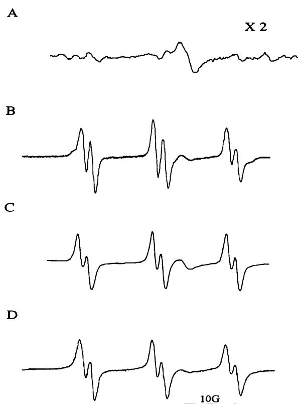
Fig 1. ESR spectra of PBN-adduct obtained in enzymatic reaction of \text{CCl}_4 in rat liver microsomes and photochemical reaction of \text{CCl}_4 ; A) in control enzymatic reaction without \text{CCl}_4 , B) in enzymatic reaction of 5 mM \text{CCl}_4 , C) in enzymatic reaction of 10 mM \text{CCl}_4 , and D) in photochemical reaction of 100 \mu l \text{CCl}_4 . PBN was 10 mM at final concentration in enzymatic reaction, and 10 mg/ml in hexane solution in photochemical reaction (Receiver gain : A) 6.3 \times 10^3 , B), C) and D) 3.2 \times 10^3 )
