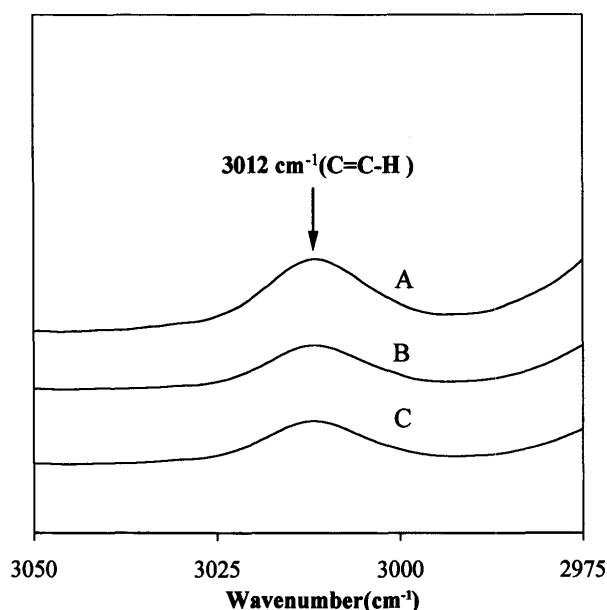
Fig 2. Infrared spectra of phospholipids in range of C-H bond in isolated -C=C-H group around 3012\text{ cm}^{-1} , A) in control enzymatic reaction without \text{CCl}_4 , B) in enzymatic reaction of 5\text{ mM CCl}_4 , and C) in enzymatic reaction of 10\text{ mM CCl}_4 .
