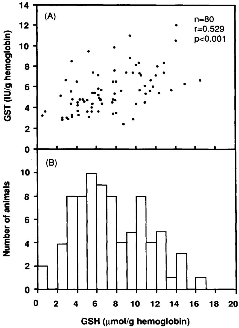
Fig. 1. The correlation between GSH content and GST activity (A), and the distribution of the GSH concentrations in sheep erythrocytes (B).
