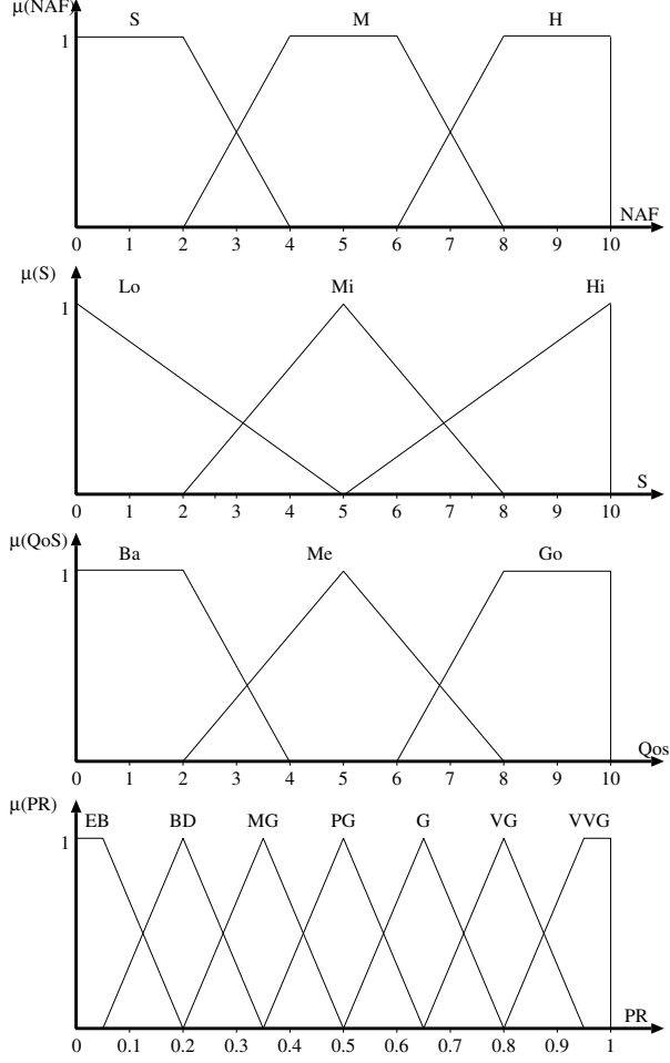
Figure 5. Membership functions.
