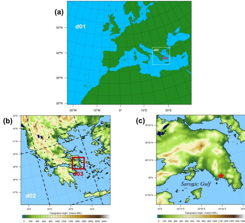
Fig. 1. Model domain configuration for: (a) the European-level parent domain (d01, 12 \times 12 km), (b) Greece domain (d02, 4 \times 4 km), and (c) Greater Athens Area (GAA) domain (d03, 1 \times 1 km). The Greece and GAA domains (red box) and associated topography are shown in 1b. The topographic map is further zoomed-in to the GAA domain (1c), with a bold red star denoting the location of the NTUA lidar site.
