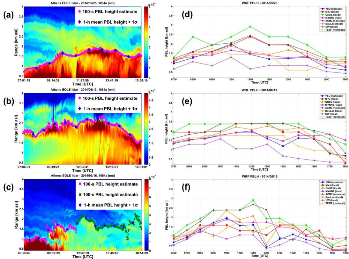
Fig. 10. Lidar range-corrected power time-range color plots (a-c) at 1064 nm wavelength and simulated PBL height from the WRF model (d-f) for; top row) Continental, middle row) Etesians, and bottom row) Saharan synoptic flow types. Lidar time-range plots are overlaid with PBL height estimates (circles, 100-s resolution) using the extended Kalman filter technique, in addition to the 1-h mean PBL height (blue diamonds) calculated with nine 100-s estimates, along with 1\sigma standard deviation.
