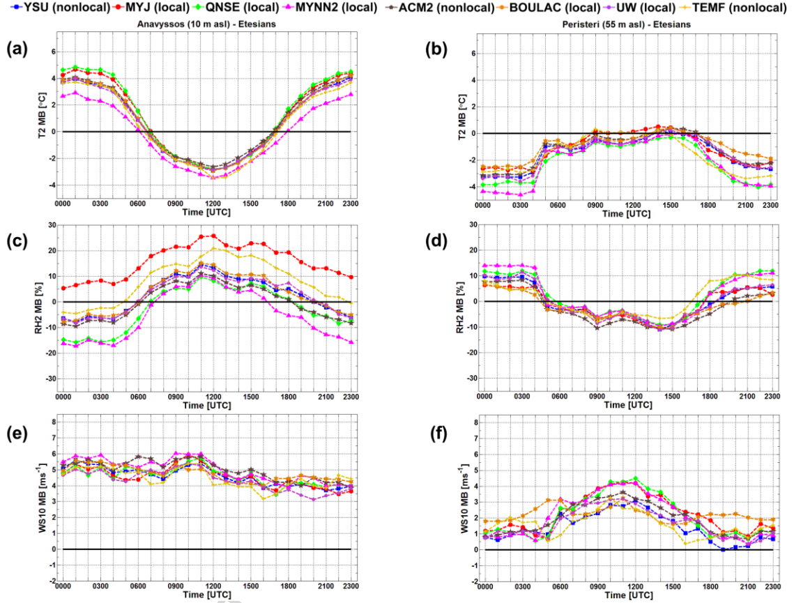
Fig. 7. Same as in Fig. 5, but time-averaged for Etesians synoptic flow days.
