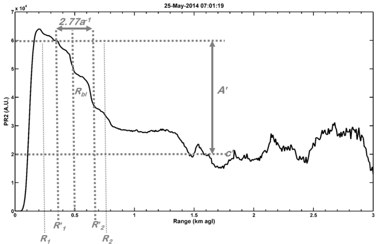
Fig. 3. 100-s profile of molecular-normalised range-corrected power from the NTUA lidar at 0701 UTC on 25 May 2014. Initial state vector [R_{bl} \ a \ A' \ c'] with lower- and upper-range limits [R_1 \ R_2] for the extended Kalman filter (EKF) PBL height technique are annotated in gray dashed lines.
