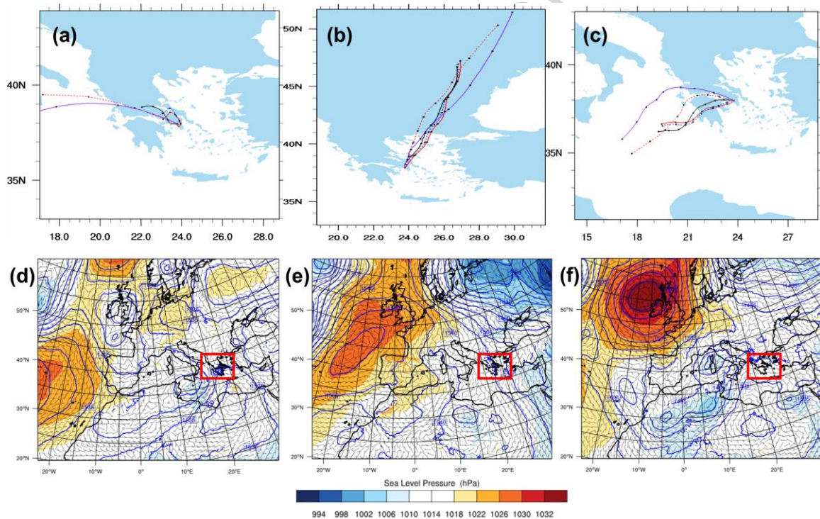
Fig. 2. Two-day FLEXPART-WRF backtrajectories (top) ending at Athens (37.96N, 23.78E) and synoptic maps simulated with the WRF model (bottom) representing (from left to right), Continental (25 May 2014), Etesians (13 June 2014), and Saharan (16 June 2014) flow types. Backward trajectories end at 1200 UTC with black dots showing 6-h position and colors denote trajectory height at receptor for 0.5 km (red), 1 km (blue dashed), 2 km (black), 3 km (red dashed), and 4 km (purple). Synoptic maps (valid 1200 UTC) show sea level pressure in hPa (coloured contours), geopotential height at 850-hPa in metres (blue lines), and 850-hPa winds (barbs).
