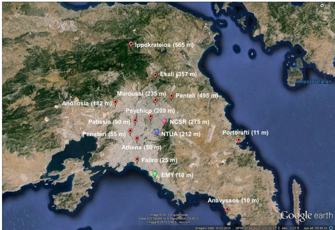
Fig. 4. Location and elevation (meters above sea level) of the 14 surface meteorological stations (12 from the National Observatory of Athens, one from NTUA, and one from NCSR), and site of radiosonde launches (EMY). Spatial variations range from 500 m – 12 km apart and in elevation from 10 – 565 m asl.
