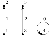
FIGURE 4. The Skolem labeling of 2\vec{K}_2 \cup \vec{L} associated to (1, 1, 2, 0, 2) .
