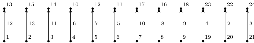
FIGURE 3. A Langford labeling of 12\overrightarrow{K_2} .
