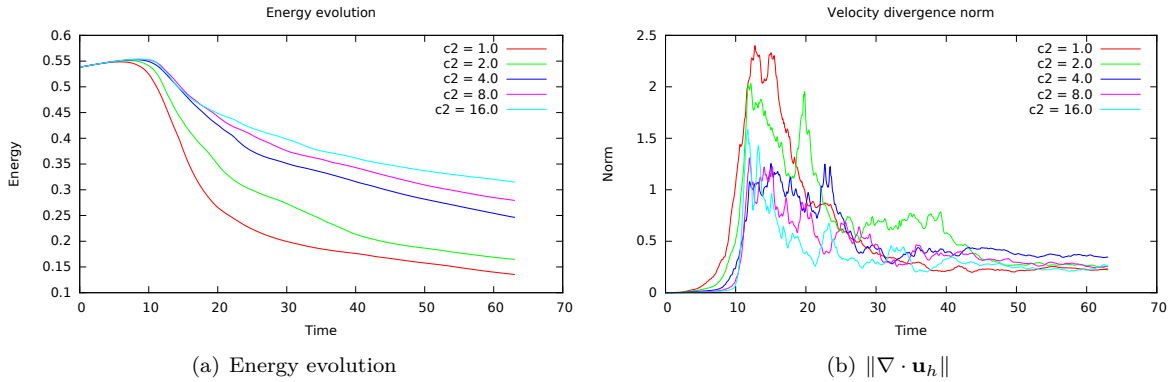
Figure 14: Energy evolution and velocity divergence norm for different values of c_2 , keeping c_1 = 12.0 and c_c = 1.0
