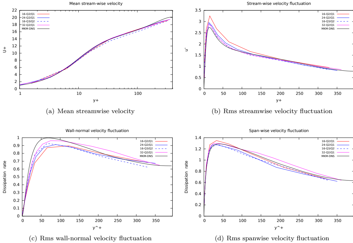
Figure 19: Mean stream-wise velocity and rms velocity fluctuations for using different discretizations.
