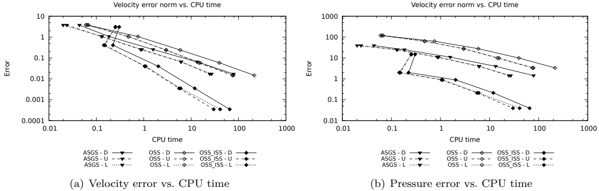
Figure 3: Colliding flow error vs. CPU time using P_U(\tilde{A}) for the global matrix.
