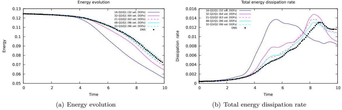
Figure 10: Energy and Total energy dissipation rate evolution refining the mesh with c_c = 4.0 .
