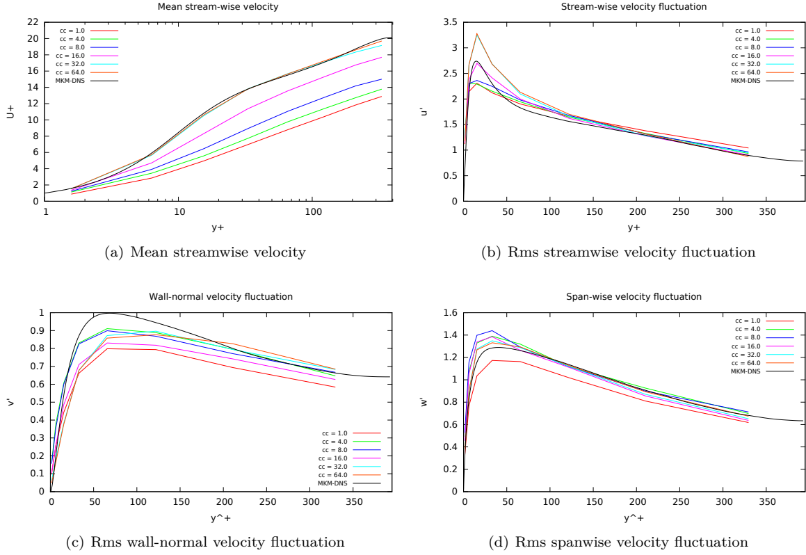
Figure 17: Mean stream-wise velocity and rms velocity fluctuations using a 16^3 Q2/Q1 mesh for different choices of c_c .
