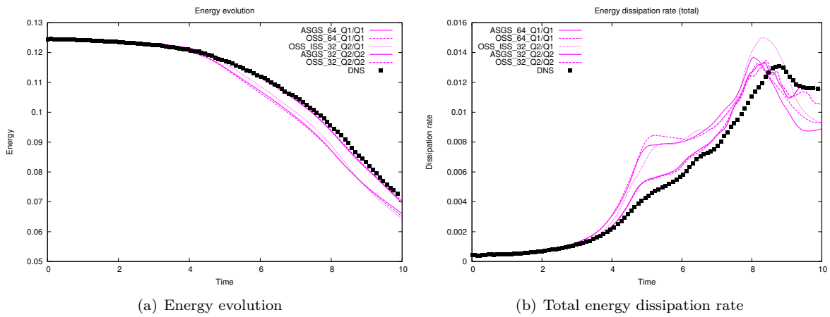
Figure 5: Energy and Total energy dissipation rate evolution with 64^3 velocity DOFs
