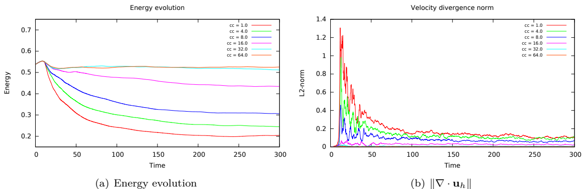
Figure 16: Energy evolution and velocity divergence norm for different values of c_c , keeping c_1 = 12.0 and c_2 = 8.0
