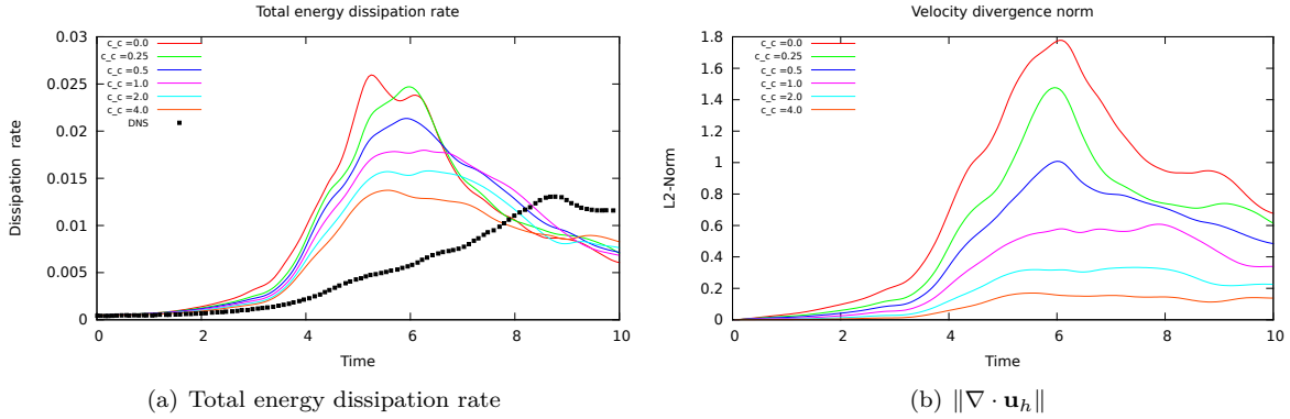
Figure 9: Total energy dissipation and velocity divergence L_2 -norm for different c_c choices for OSS-ISS with 32^3 velocity DOFs
