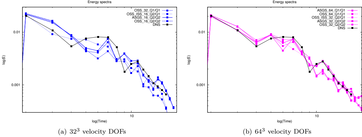
Figure 6: Energy spectra at t = 9.0
