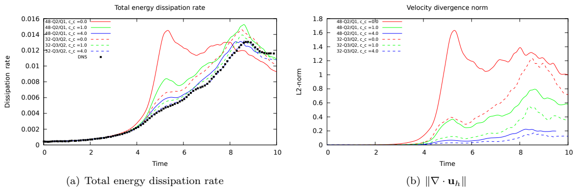
Figure 12: Total energy dissipation and velocity divergence L_2 -norm for different c_c choices for OSS-ISS with 96 3 velocity DOFs
