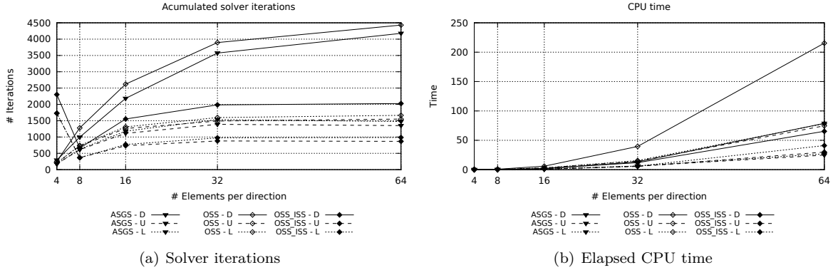
Figure 1: Colliding flow solver iterations and elapsed CPU time using P_U(\tilde{\mathbb{A}}) for the global matrix.
