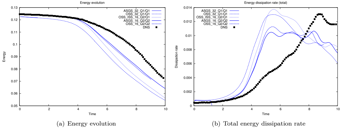
Figure 4: Energy and Total energy dissipation rate evolution with 32^3 velocity DOFs
