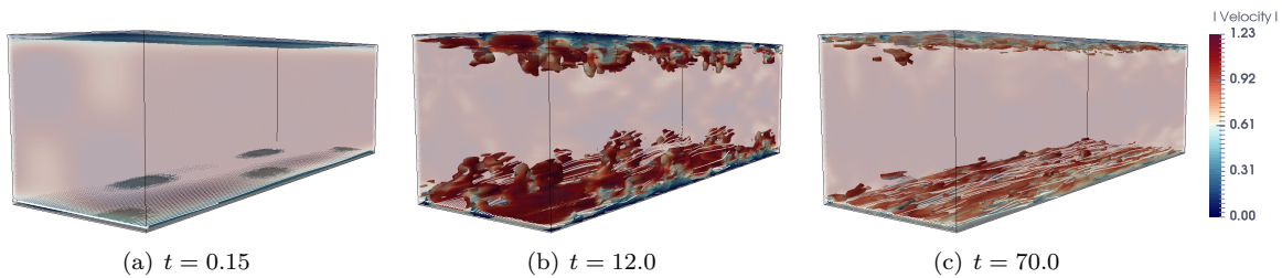
Figure 15: Velocity module at different times with c_1 = 12.0 , c_2 = 1.0 and c_c = 32.0 using a 32^3 Q2/Q1 elements mesh.
