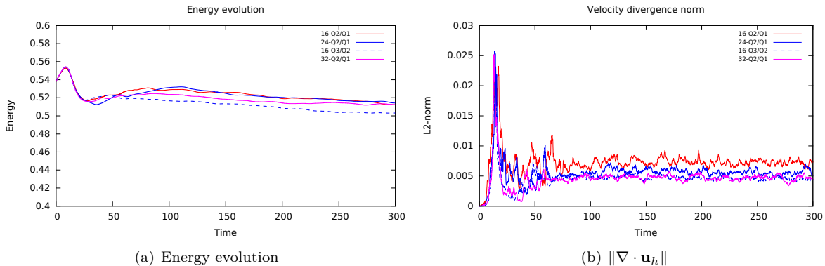
Figure 18: Energy evolution and velocity divergence norm refining the mesh, keeping c_1 = 12.0 , c_2 = 8.0 and c_c = 32.0
