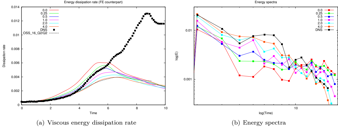
Figure 8: Comparison for different c_c choices for OSS-ISS with 32^3 velocity DOFs
