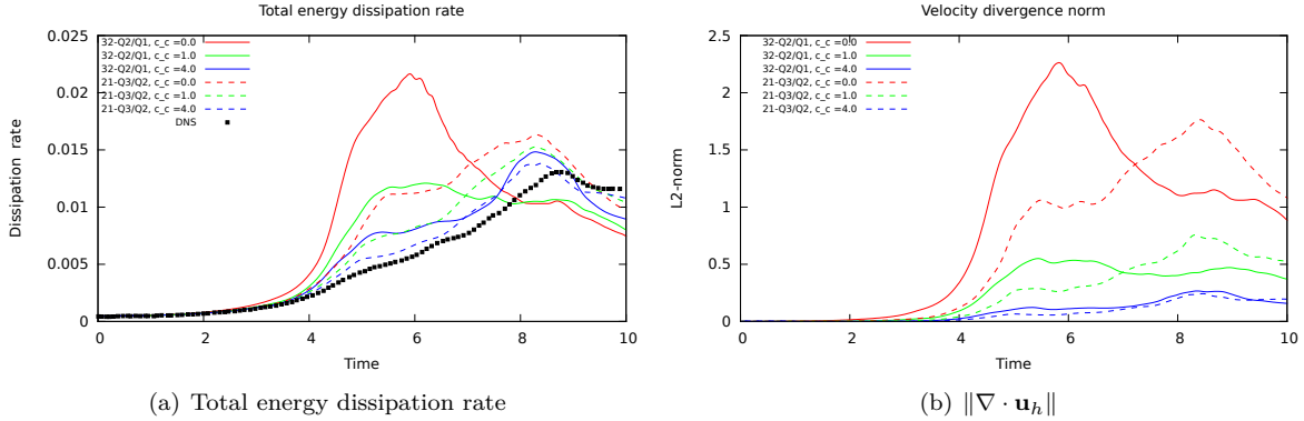
Figure 11: Total energy dissipation and velocity divergence L_2 -norm for different c_c choices for OSS-ISS with 64^3 velocity DOFs
