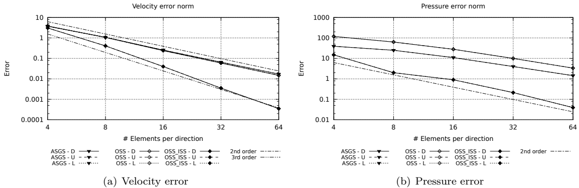
Figure 2: Colliding flow error convergence using P_U(\tilde{\mathbb{A}}) for the global matrix.
