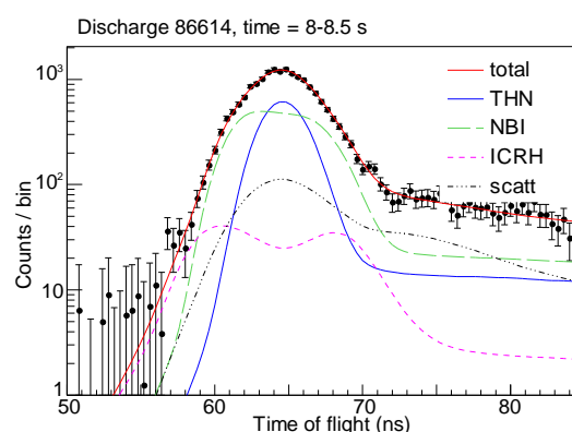
Figure 5 TOFOR data points with error bars for discharge 86614 integrated over a time interval of t = 8 -8.5 s. Also fitted components describing thermonuclear (TH), NBI, ICRH and scattered neutrons are shown.
