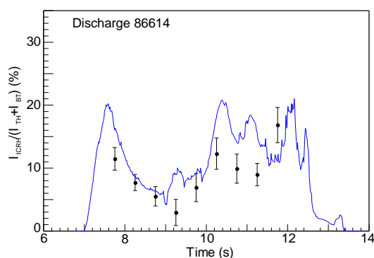
Figure 4 Enhancement of the neutron rate due to second harmonic D damping according to PION (blue line) and TOFOR (points with error bars) for discharge 86614.
