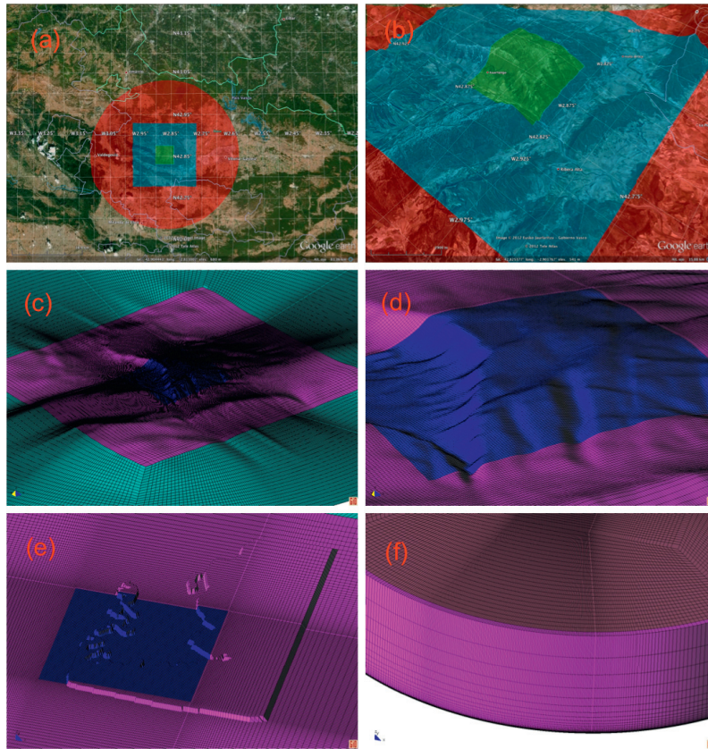
Fig. 1. Example of WindMesh output. (a) and (b) show the buffer (red), transition (blue), and farm (green) zones as seen in GoogleEarth. (c) y (d) surface mesh at the different zones. Topography has been smoothed. (e) roughness contours interpolated from a map file. (f) detail of the 3D mesh.
