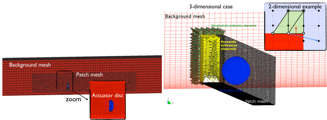
Fig. 2. Left: Example to illustrate the Chimera concept in wind farm modeling. A patch mesh contains the actuator disc, represented by a body-fitted mesh, and eventually local refinement downstream. Note that the interior of the disk is also solved so that the mesh covers both the exterior and interior parts of the rotor. Right: Example of the extension elements used to connect patch and background meshes. A brick patch meshed with tetrahedral (pyramids) elements contains the actuator disk (shown in blue) and interfaces with a background structured mesh of hexahedral elements. For clarity, the inset shows a simpler 2D example of extension elements.
