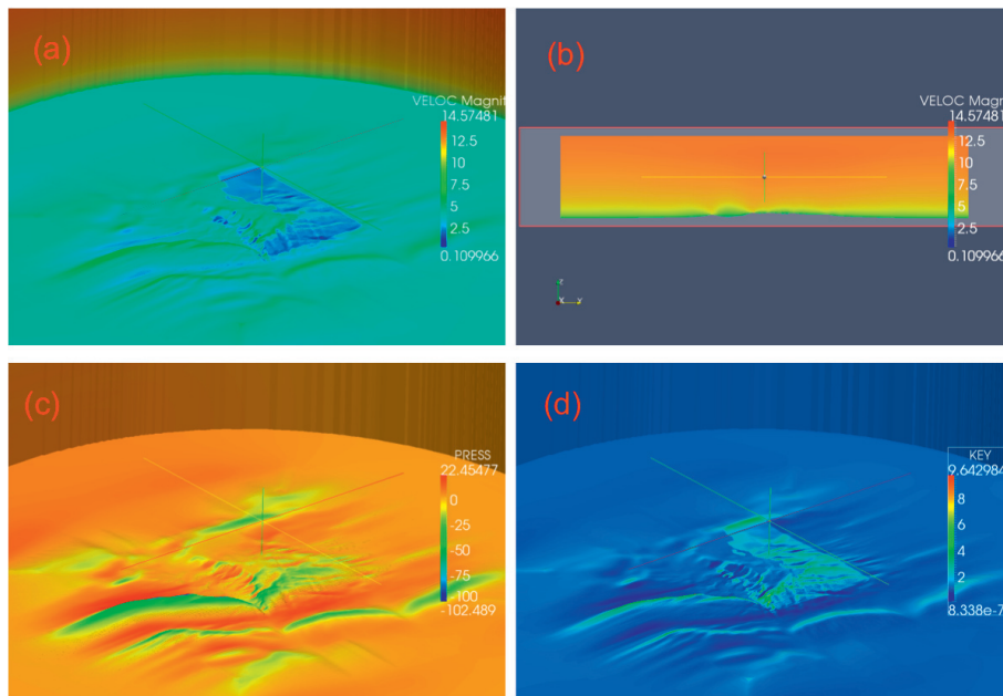
Fig. 5. Results for ABL simulations of a wind farm in Spain. (a) wind speed at surface. (b) Wind velocity in a vertical cut along the inflow wind direction. (c) pressure at surface. (d) turbulent kinetic energy at surface.
