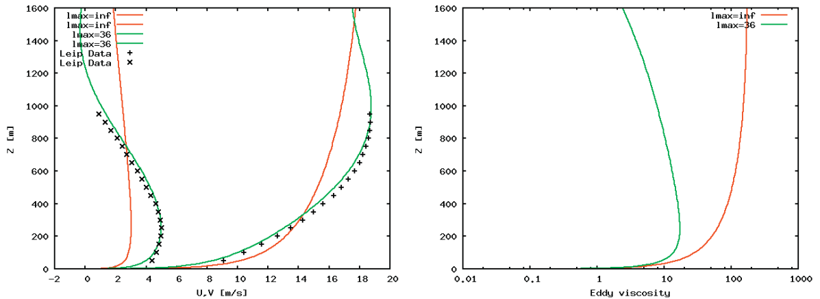
Fig. 3. Vertical profiles of wind velocity components (left) and eddy viscosity (right) using the standard k - \epsilon model (i.e. l_{max} \rightarrow \infty ) and the ABL k - \epsilon model modified by limiting the mixing length as explained in section 2.2.1 ( l_{max} = 36\text{m} in this case). Note how the second option improves substantially the fits to the experimental Leipzig profile data, indicated by crosses.
