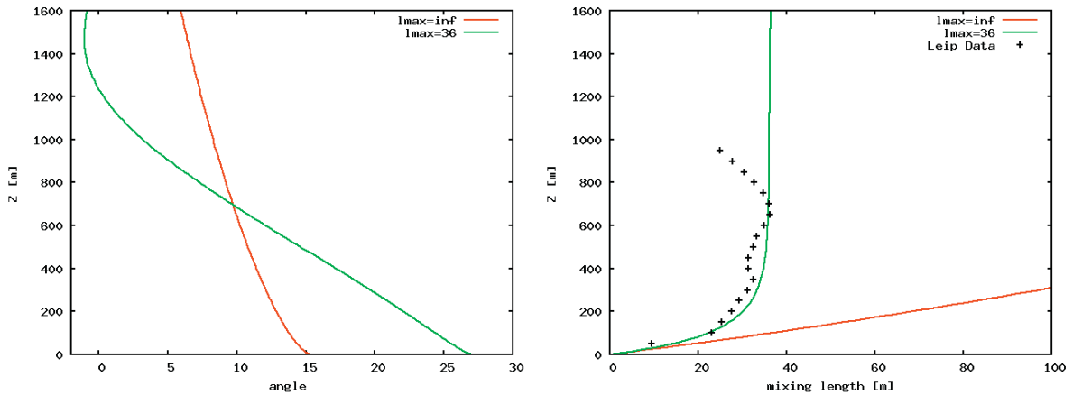
Fig. 4. Vertical profiles of wind turning angle ( \alpha = 0^\circ at z = 3000\text{m} ) and mixing length profiles using the standard k-\varepsilon model (i.e. l_{max} \rightarrow \infty ) and the ABL k-\varepsilon model modified by limiting the mixing length as explained in section 2.2.1 ( l_{max} = 36\text{m} in this case). Experimental measurements showed a surface wind turned by 26.1^\circ from the geostrophic and a friction velocity of u_* = 0.65\text{ m/s} . The standard k-\varepsilon predicts too large friction velocity u_* = 0.81\text{ m/s} whereas the limited length model predicts u_* = 0.676\text{ m/s} . The surface wind is turned only 15^\circ when using the standard k-\varepsilon model and 27^\circ when using the mixing length correction, in excellent agreement with measurements.
