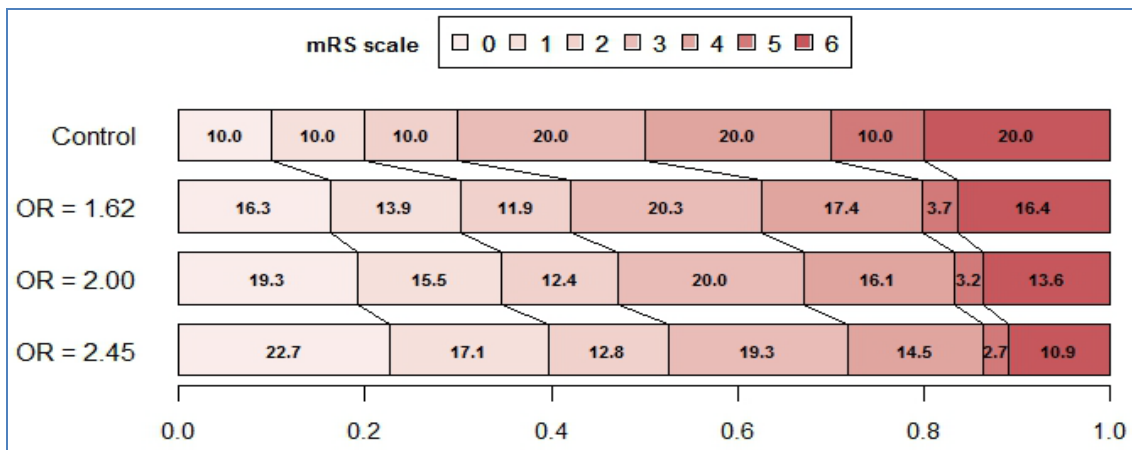
Figure 3: In scenario C , again, the same OR applies to the first 5 cut-points and it is diluted in the last 5 to 6 frontier; but now the common averaged OR results in an estimate of 1.62; 2.00 and 2.45.
