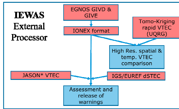
Figure 5: Layout of the Ionospheric EGNOS Warning System (IEWAS).
