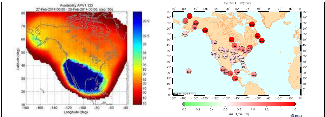
Figure 4. WAAS APV-1 availability (top) and AATR index computed for WAAS Reference Stations on the same day (27/02/2014) at hour 22-23 UT.
