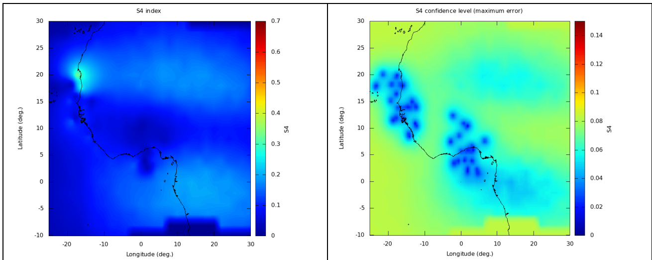
Figure 12 : Scintillation maps (S4 level) and corresponding confidence level over West Africa using data from Dakar and Lomé.
