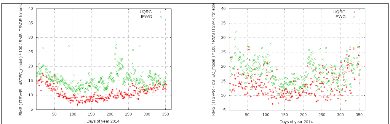
Figure 8: dSTEC relative assessment during 2014, of EGNOS-IEWAS (green) and UPC-UQRG (red) VTEC models, for one high-latitude and one mid-latitude IGS European GNSS receivers: ONSA (E11.9°,N57.2°) –left- and EBRE(E0.5°,N40.6°) –right-
