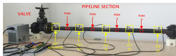
Figure 6 Experiment configuration
