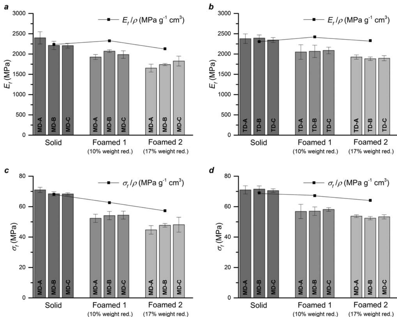
Figure 4. (a) Flexural modulus of samples tested in MD direction; (b) Flexural modulus of samples tested in TD direction; (c) Flexural strength of samples tested in MD direction; (d) Flexural strength of samples tested in TD direction. Solid line in graphs represents specific flexural properties.
