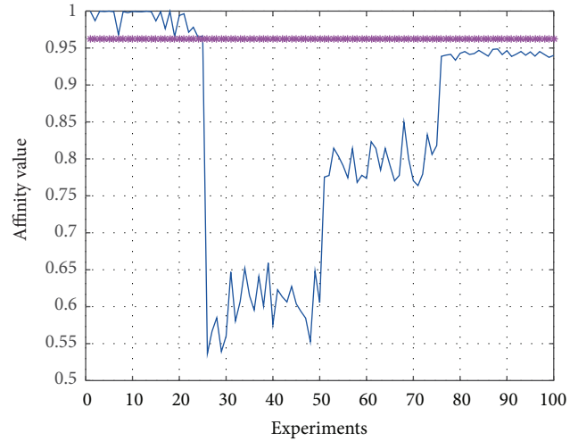
FIGURE 13: Affinity values between a memory cell of the memory cell set of the healthy state (MCSH) and the data coming from the structure to diagnosis (phase 4).
