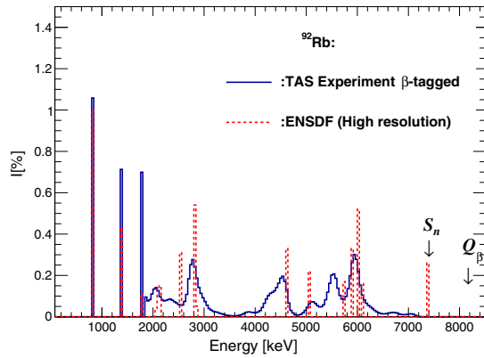
FIG. 2 (color online). Beta intensity for the decay of ^{92}\text{Rb} obtained with TAS measurements in the blue continuous line. Red dashed lines are data from ENSDF [19]. Ground state feeding from ENSDF is 95.2\% \pm 0.7\% , while from this work it is 87.5\% \pm 2.5\% .
