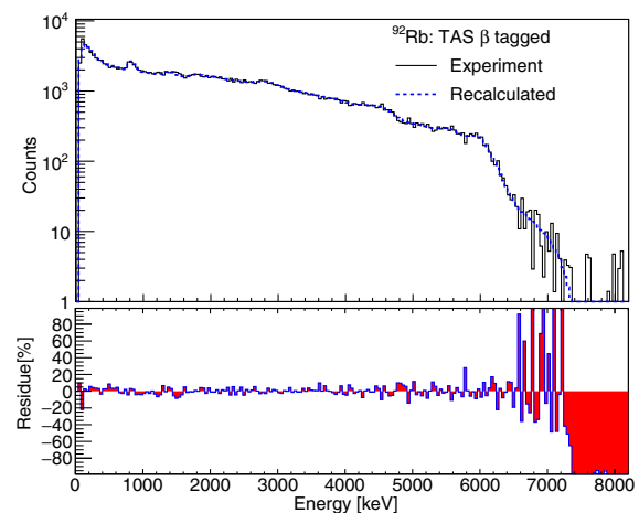
FIG. 1 (color online). Upper panel: Comparison between measured spectrum (black continuous line) and reconstructed one (blue dashed line) with the feeding obtained from the TAS data analysis. Lower panel: Residues between the two curves reported in the upper panel.
