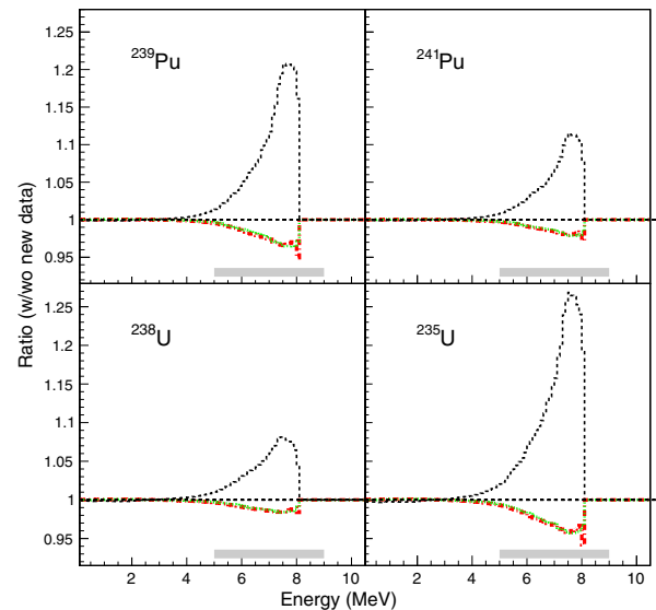
FIG. 3 (color online). Ratio between the antineutrino spectra calculated using the results presented in this Letter with respect to the data on ^{92}\text{Rb} decay used in Ref. [12] (thick red dashed-dotted line), in Ref. [40] (green dotted line), and in Ref. [41] (black dashed line). The sharp drop in the ratio, in one single bin located at the Q value of the ^{92}\text{Rb} , is due to the different values in Q given in Refs. [16] and [19], that were used to reconstruct the antineutrino spectrum. A gray horizontal bar is placed above the antineutrino energy scale to indicate the region of the distortion observed by the reactor antineutrino experiments with respect to the converted spectra.
