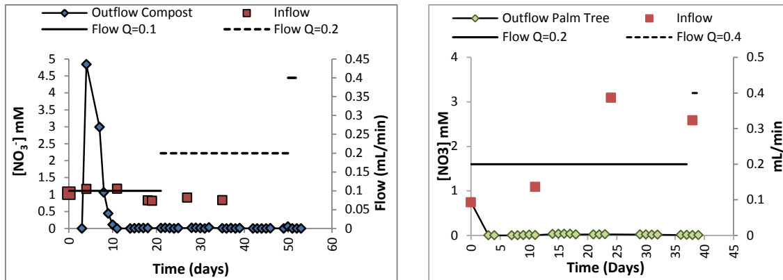
Figure 2. Nitrate concentration in the inflow (squares) and outflow water (diamonds) of the compost column and palm tree experiments.
