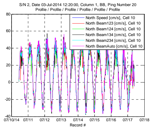
Fig.4 Slightly diverging currents for four beam and three beam solutions.
