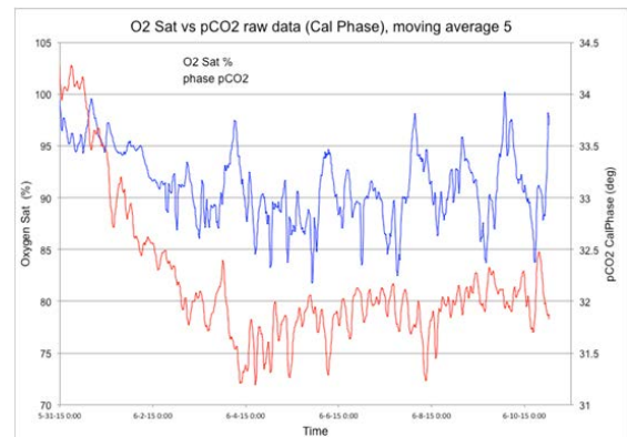
Fig. 10. Oxygen and pCO 2 data from a 10 days deployment in June 2015
