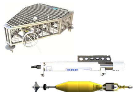
Figure 1. Scheme of the equipment: Obsea, CTD and buoy of the right to left
