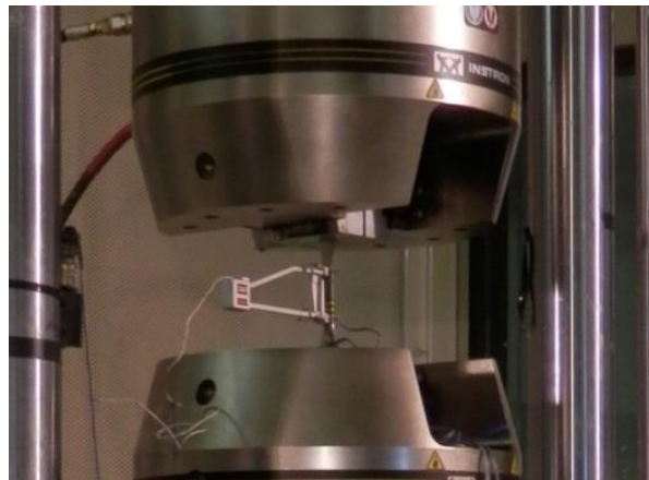
Figure 3. Coupon in INSTRON tensile testing machine.
