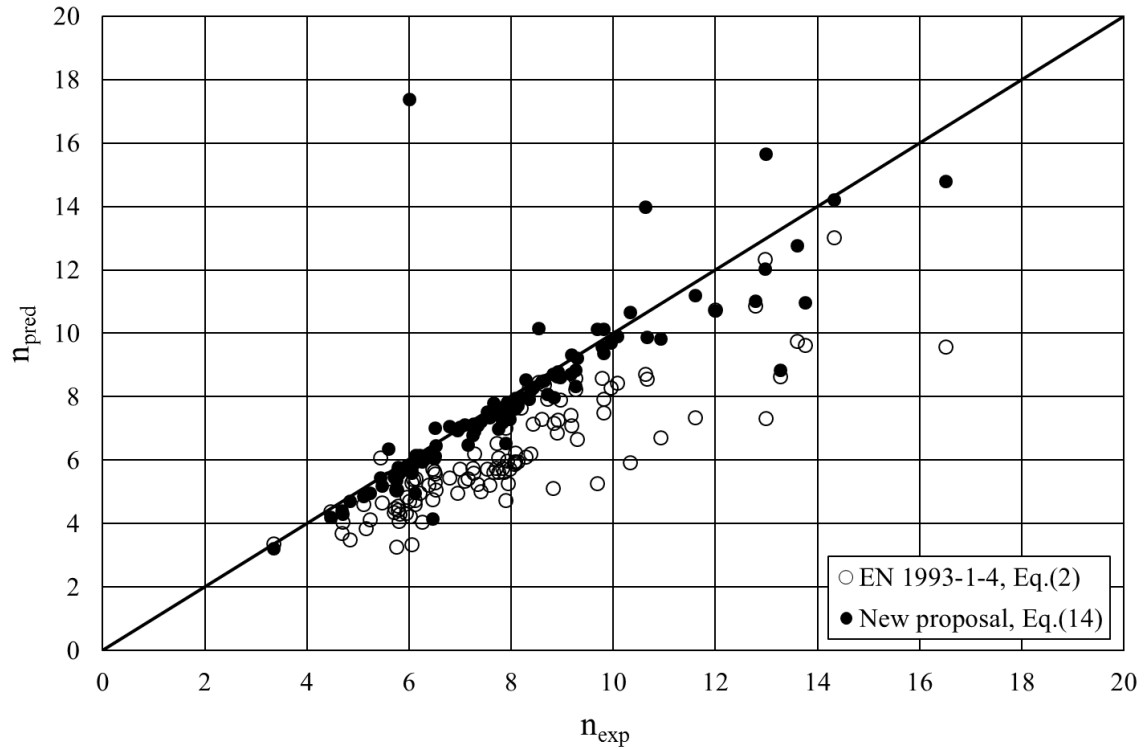
Figure 11. Prediction of strain hardening parameter n for duplex and lean duplex stainless steels.
