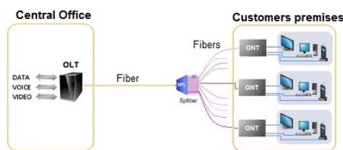
Fig.2.2: Typical PON network architecture.
