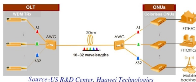
Fig.2.3: Typical WDM-PON architecture [4].
