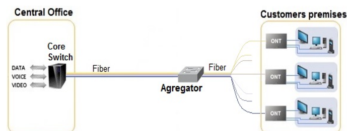
Fig. 2.4: AON typical Architecture.
