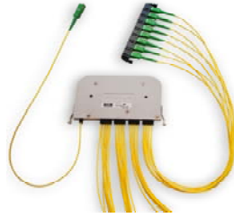
Fig. 4.13. RDJ 901 200 Optic Splitter.
