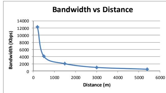
Fig.1.3: ADSL bandwidth vs. distance
