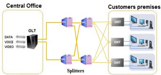
Fig.2.7: Redundant trunk and branches.
