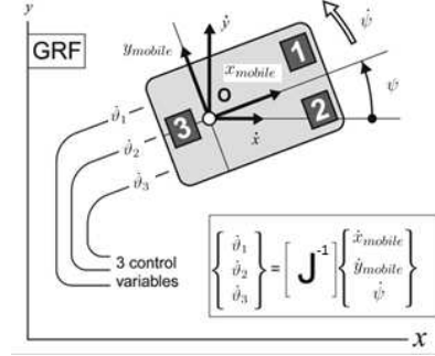
Figure 8.3: Platform position is described by means of Cartesian coordinates x and y , while its orientation is represented by the angle \psi .
