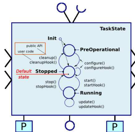
Figure 6.6: TaskContext's states
