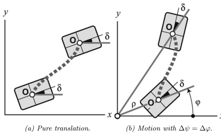
Figure 8.4: Holonomic movements.
