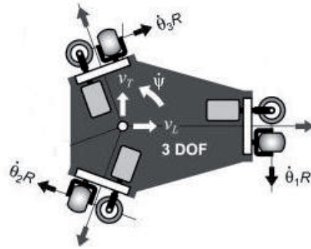
Figure 5.4: Previous developed platform
