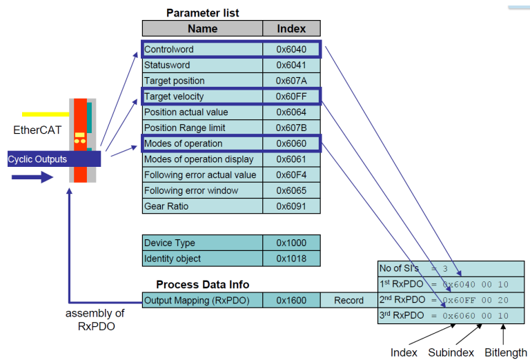
Figure A.8: An example of RxPDO mapping
