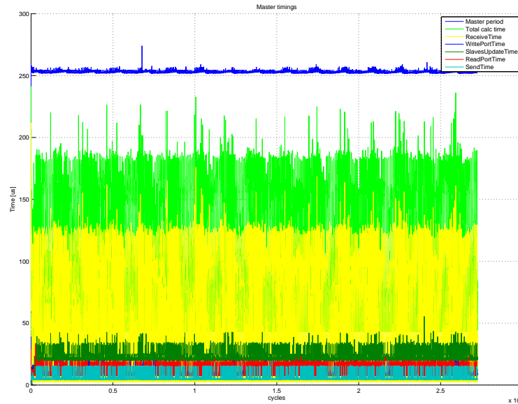
Figure 11.1: EtherCAT Master time evaluation
