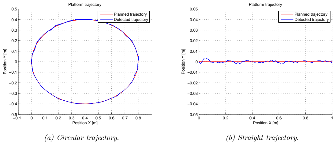
Figure 11.2: Planned and “detected” trajectories using the adaptive controller.
