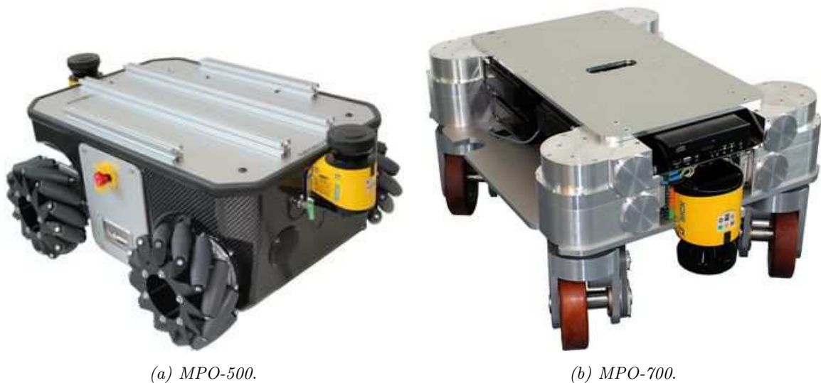
Figure 2.3: NEOBOTIX platforms
