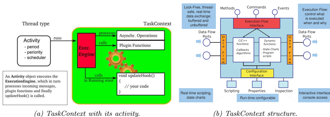
Figure 6.4: TaskContext representation
