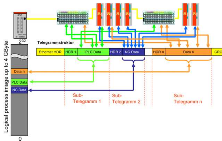
Figure A.2: EtherCAT logical addressing
