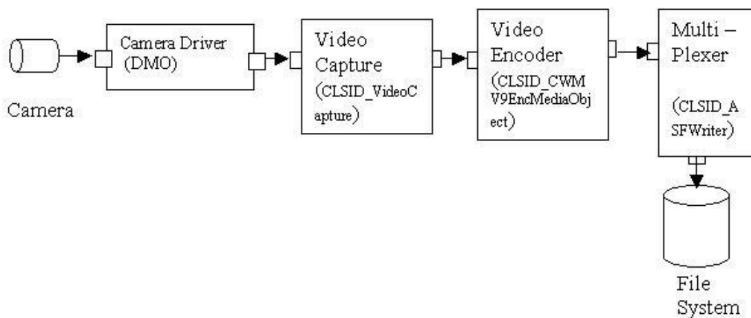
Figure 3.5 – Filter graph Capture
