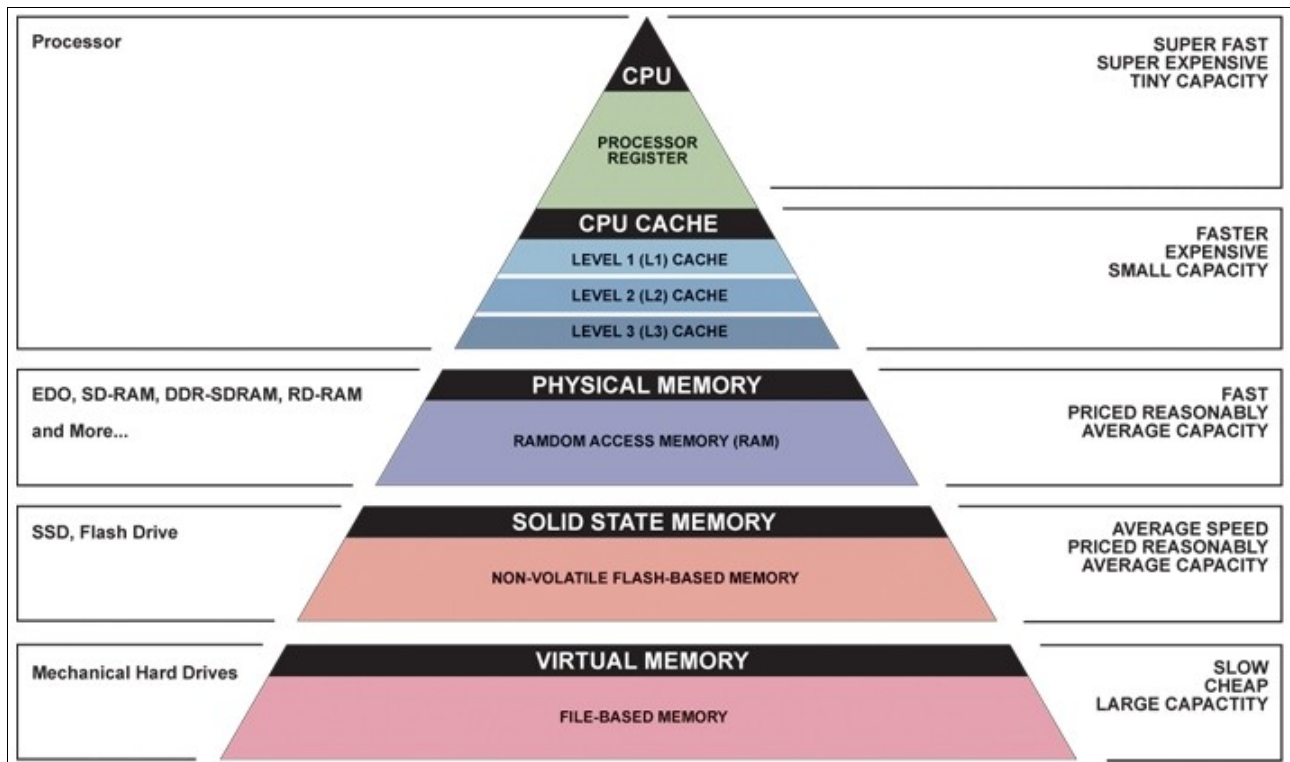
Figure 7.1 – Memory hierarchy 7
