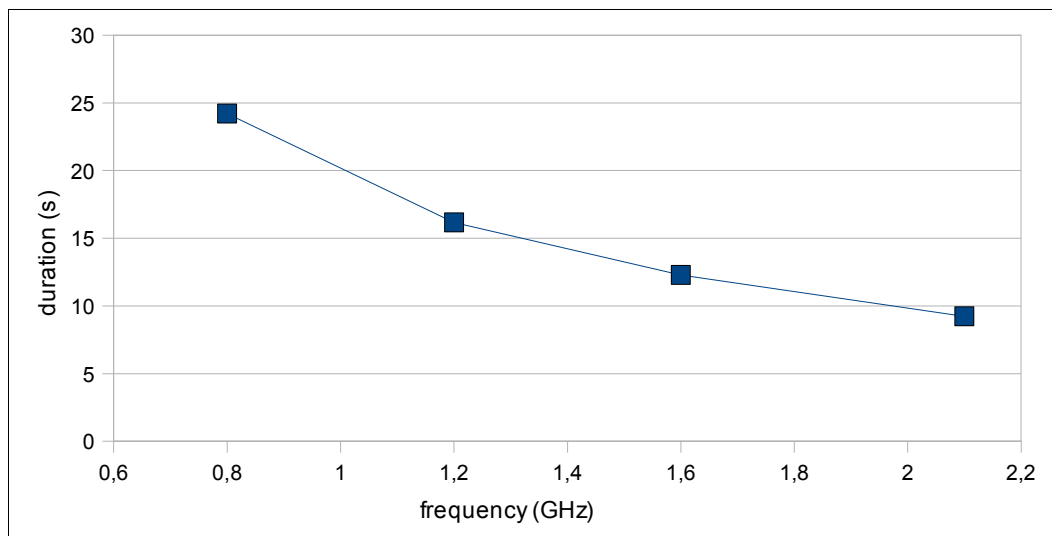
Figure 6.2 – Results of the execution times of one job with frequency scaling
