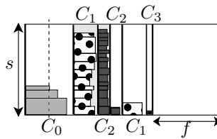
Figure 2: Packing small items into S .
