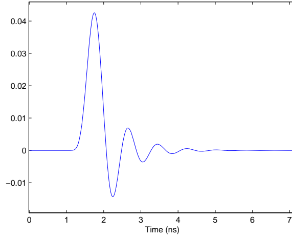
FIGURE 3.1: UWB Pulse
