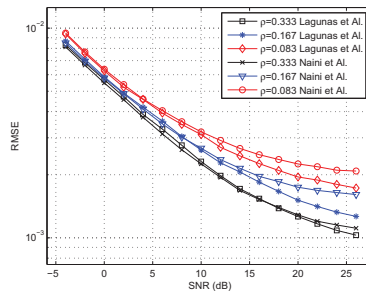
Fig. 6. RMSE of the recovered signal compared with the approach in [6]
