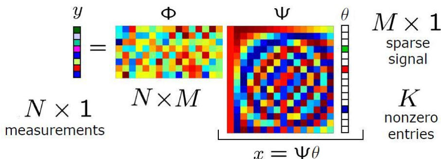
FIGURE 2.1: Compressed Sensing: Mathematical Representation
