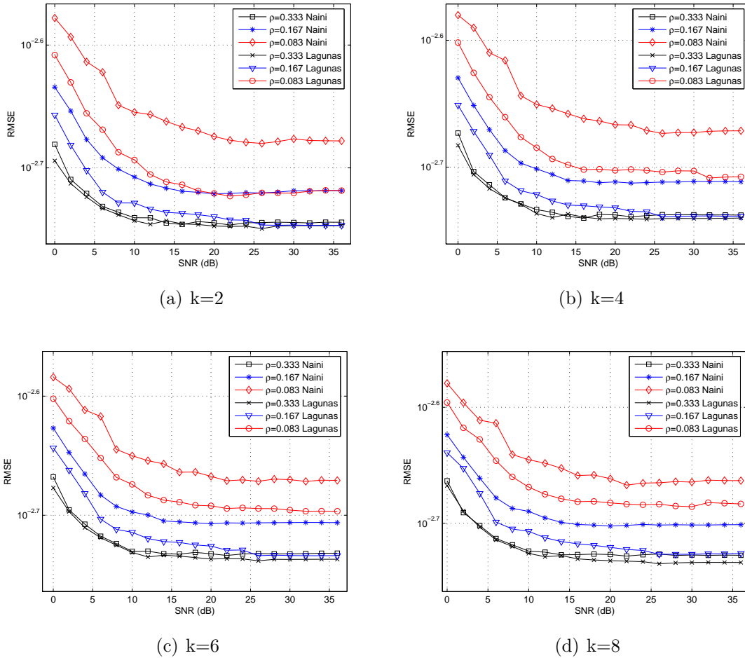
FIGURE 4.26: RMSE of the recovered signal. Comparison between the proposed model and [2] using eOMP
