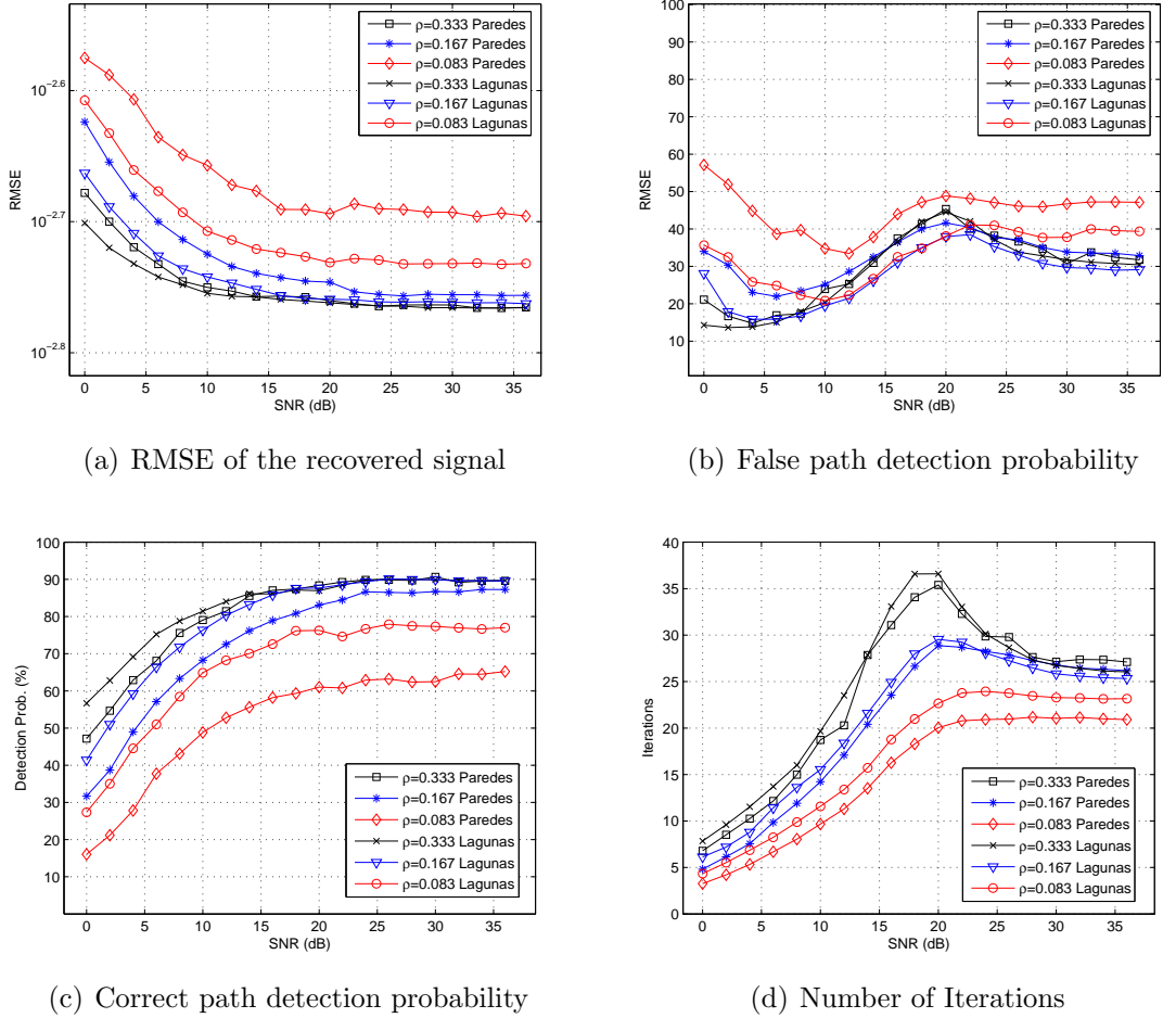
FIGURE 4.14: Comparison between the proposed model and [1] using OMP
