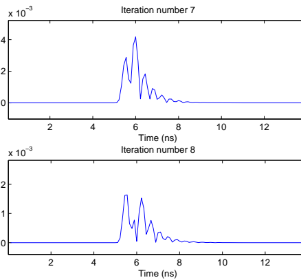
FIGURE 4.6: Received Residual Signal (2): Zoom of Fig. 4.5 at the area of interest
