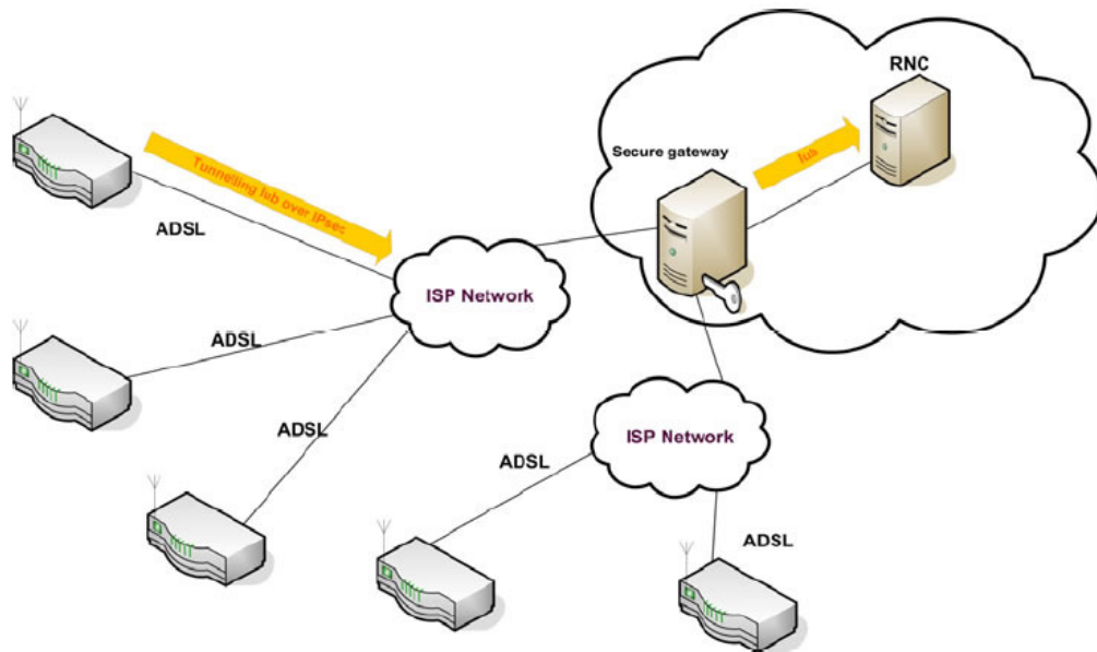
Figure 4.4. Tunnelling lub with modified RNC. [7]
