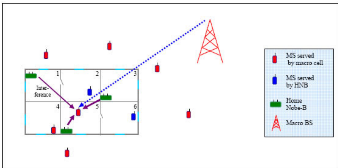
Figure 4.10. Interference case 2 setup. [49]
