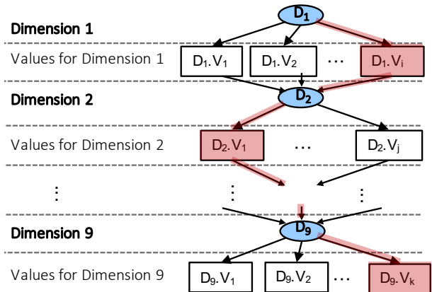
Fig. 4: Decision tree representation of reasoning knowledge.
